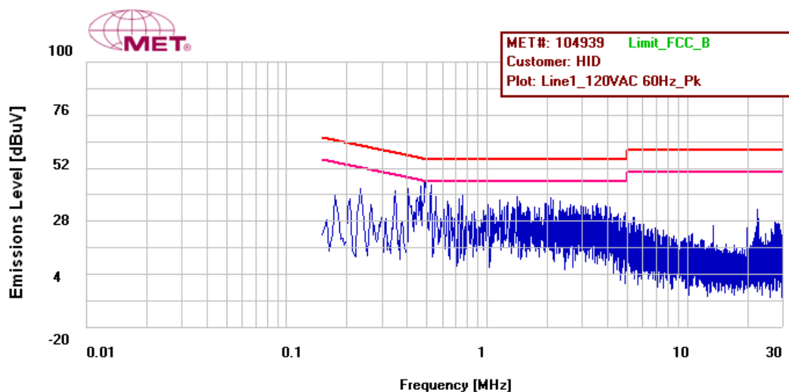
Figure 30: Conducted Emissions Limits, Terminal, Phase Line, Prescan
