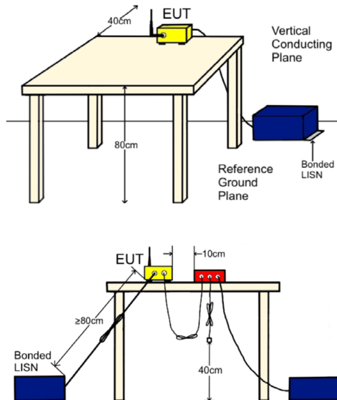
Figure 24: CEV Test Setup
