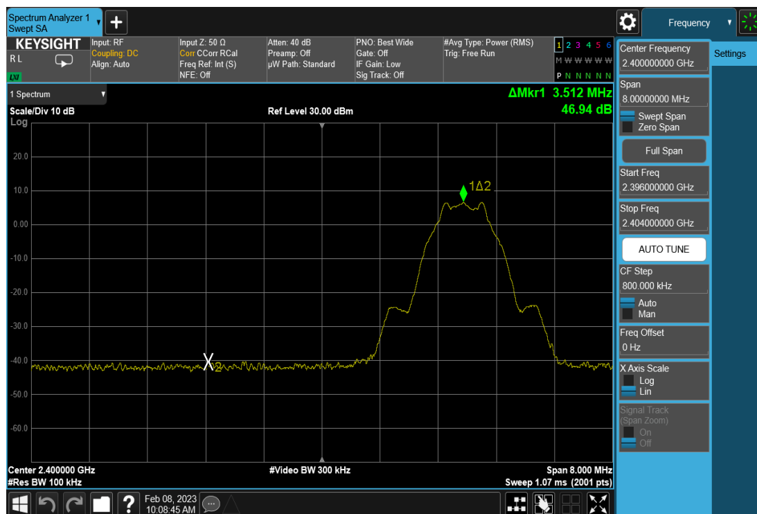
Plot 7-13. Band Edge Plot (Bluetooth (LE), 1Mbps – Ch. 0)
