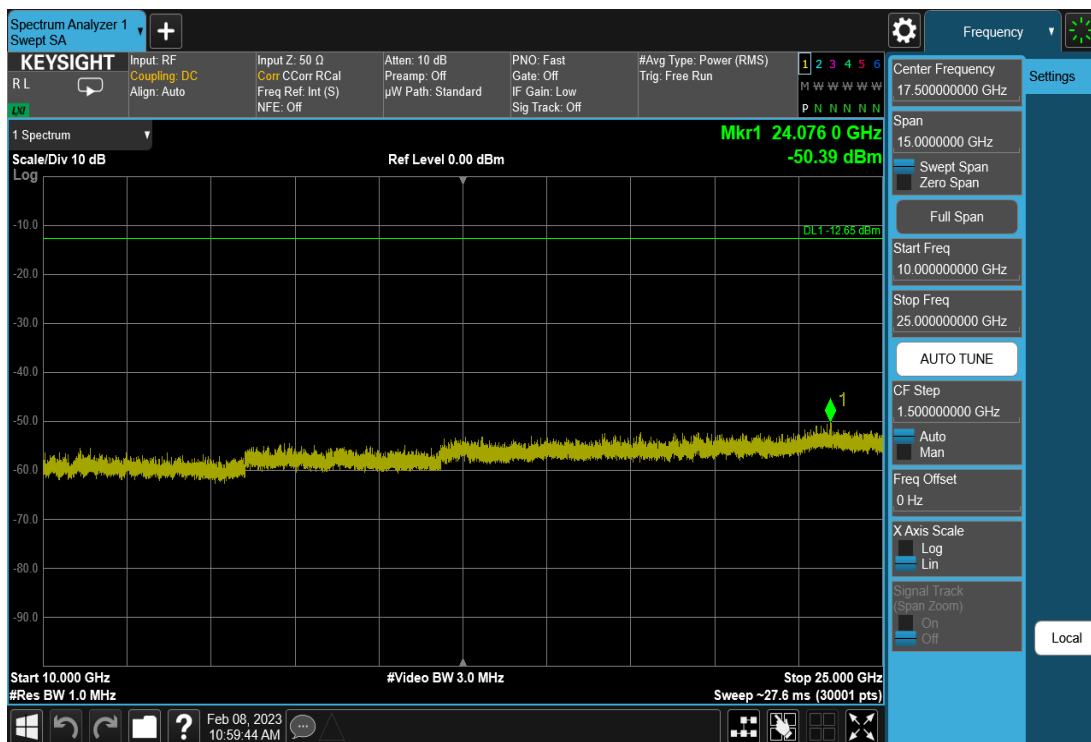
Plot 7-18. Conducted Spurious Plot (Bluetooth (LE), 1Mbps – Ch. 0)
