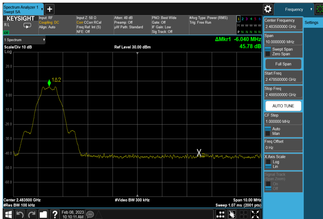
Plot 7-14. Band Edge Plot (Bluetooth (LE), 1Mbps – Ch. 39)
