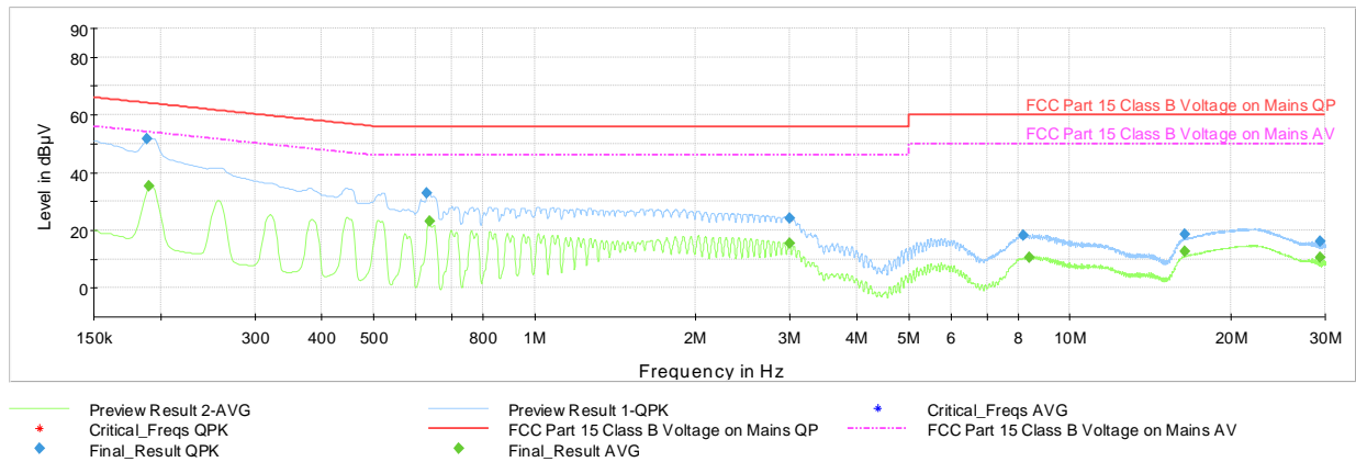
Plot 7-34. AC Line Conducted Plot with Bluetooth LE (N, 1Mbps – Ch.39, with Laptop)
