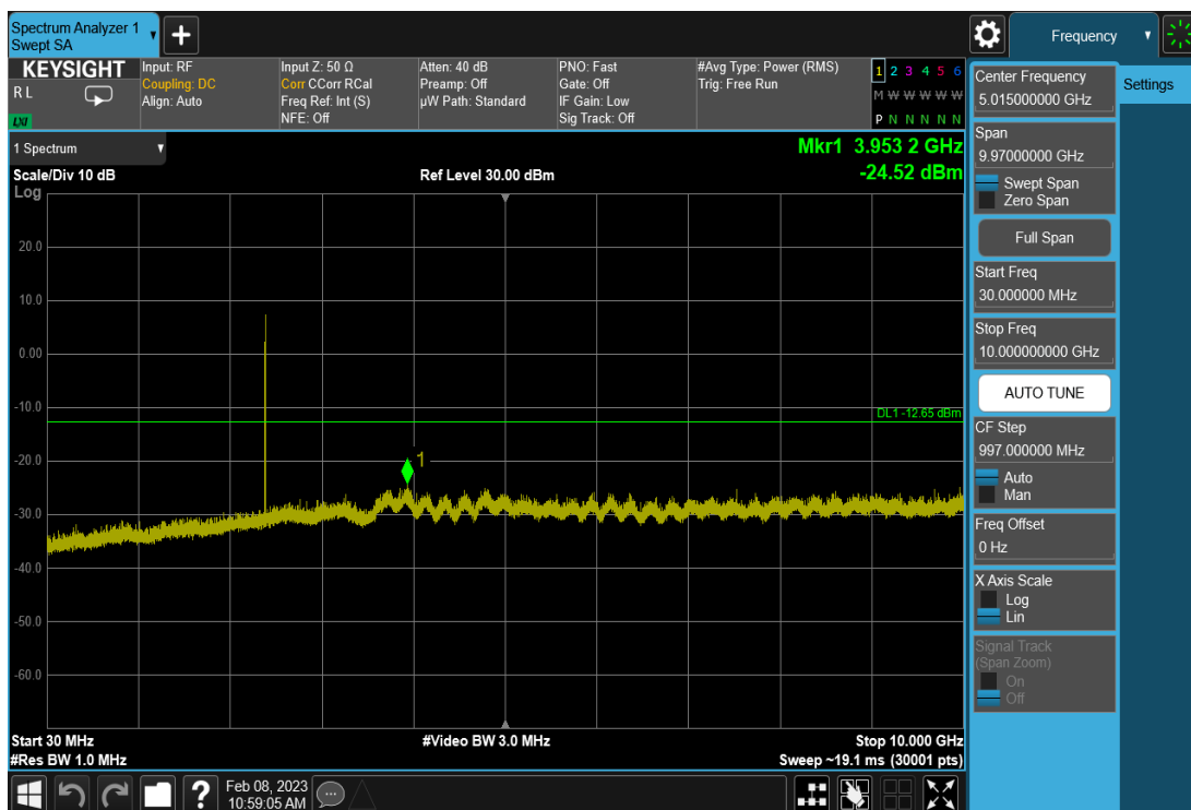
Plot 7-17. Conducted Spurious Plot (Bluetooth (LE), 1Mbps – Ch. 0)
