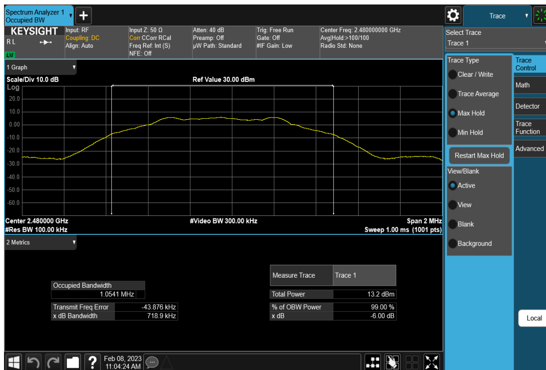
Plot 7-3. 6dB BW & 99% OBW Plot (Bluetooth (LE), 1Mbps – Ch. 39)
