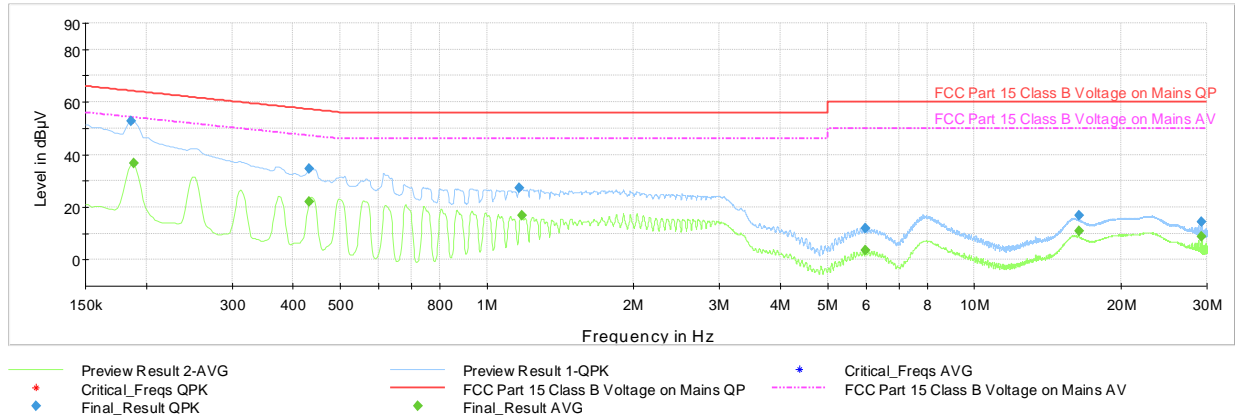
Plot 7-33. AC Line Conducted Plot with Bluetooth LE (L1, 1Mbps – Ch.39 with Laptop)
