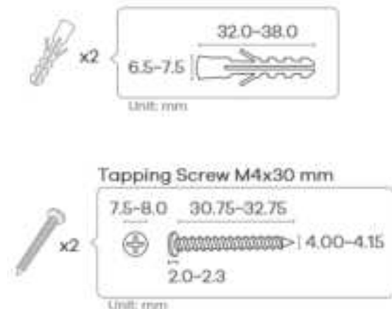
Figure 16 The WX3401 Screw Specifications
