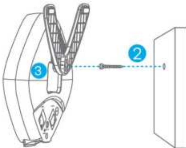
Figure 21 Wall Mounting
