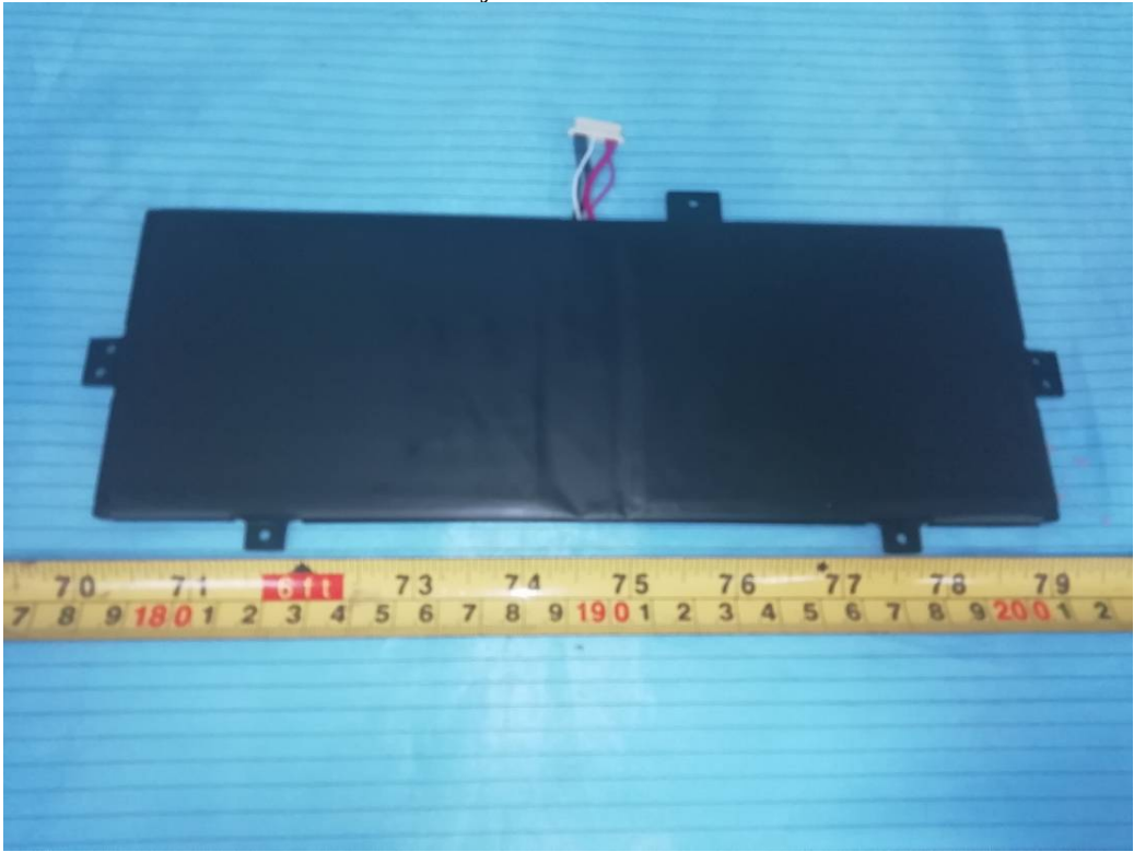
Battery: UTL-4678108-2S
