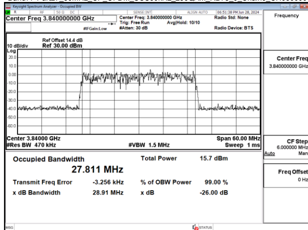
Band77-Part27_30MHz_CP_OFDM_SCS30kHz_256QAM_RB78_0_Chain0_CH656000
