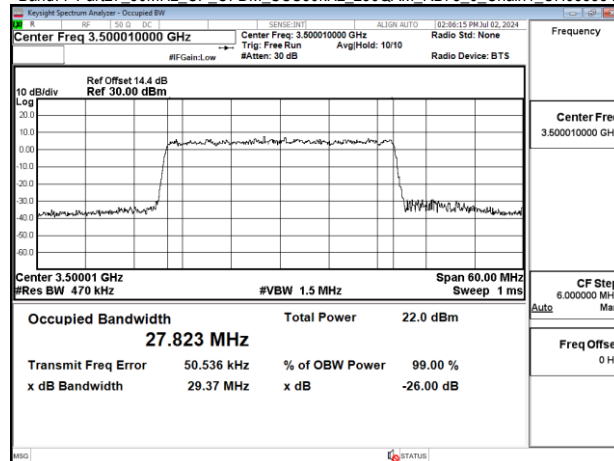
Band77-Part27_30MHz_CP_OFDM_SCS30kHz_256QAM_RB78_0_Chain1_CH633334
