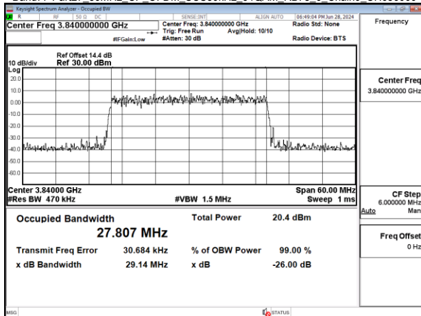
Band77-Part27_30MHz_CP_OFDM_SCS30kHz_64QAM_RB78_0_Chain0_CH656000
