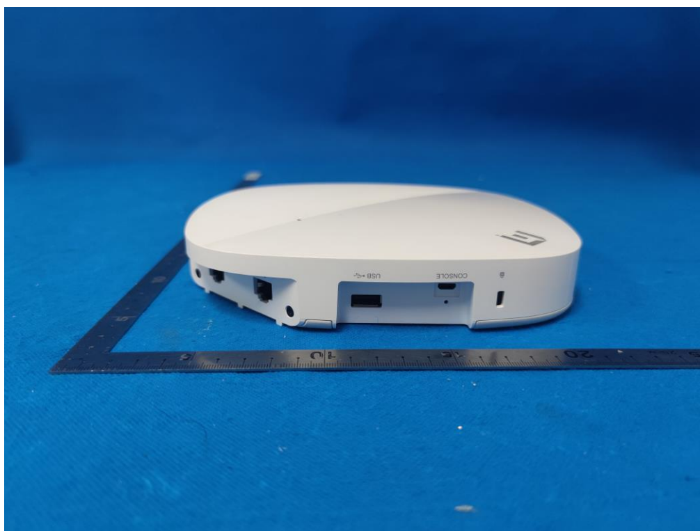
(6) EUT Photo(AP410C)
