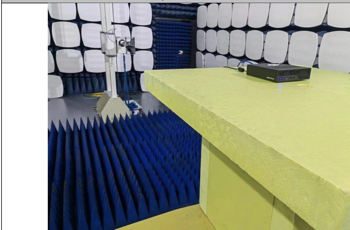
Radiated Spurious Emission, Above 1GHz
