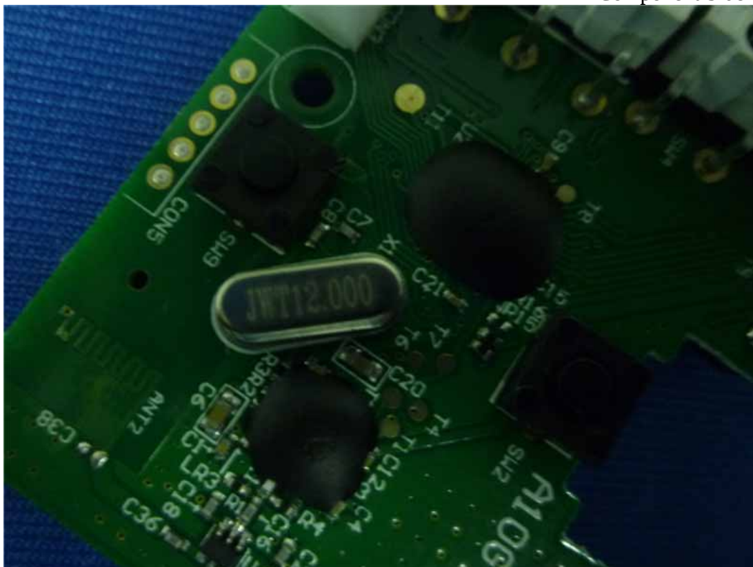
Figure 12 Component Side of the PCB
