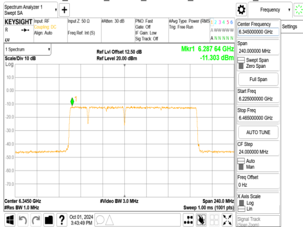
802.11be_160MHz_ChainB_6345MHz_996+484+242_MR5
