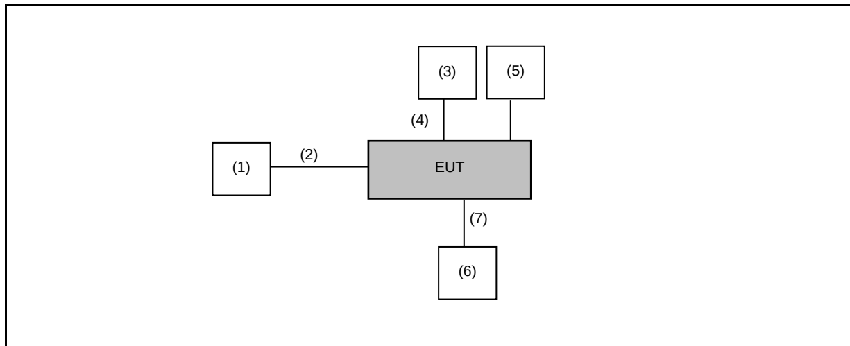
Conduction Emission
