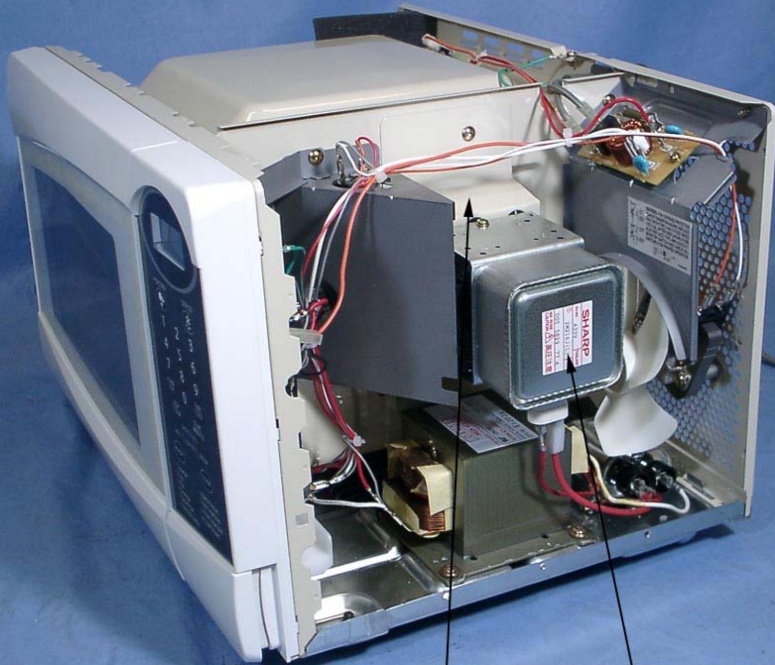
Waveguide
