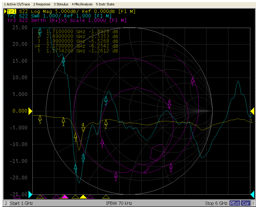
ANT3
