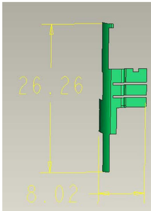
ANT8
