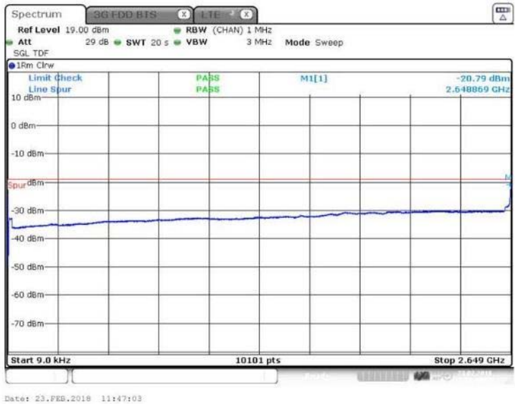
Figure 71 Spurious Emissions (9kHz – 2.649 GHz) – QPSK (2655 MHz, 10 MHz Channel BW)
