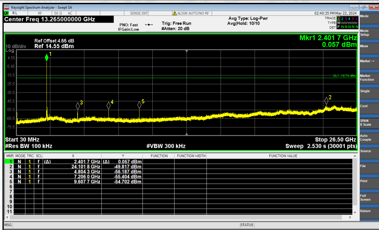
Tx. Spurious NVNT 2-DH1 2402MHz Ant1 Emission
