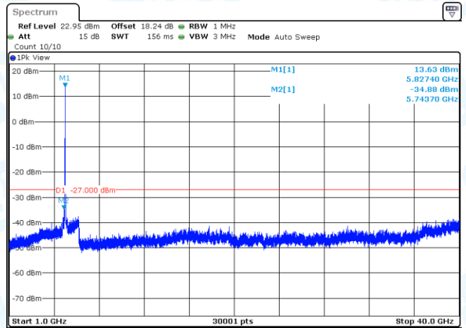
11AC20SISO-Ant1-5785-1000~40000-PASS
