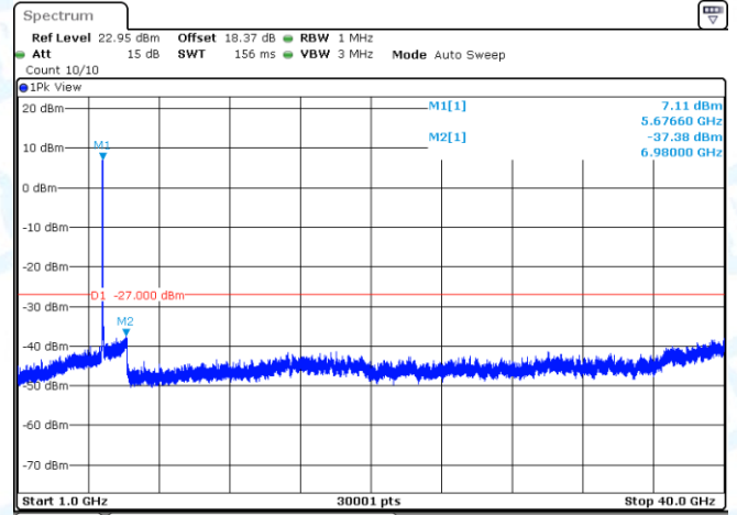
11AC40SISO-Ant1-5670-1000~40000-PASS
