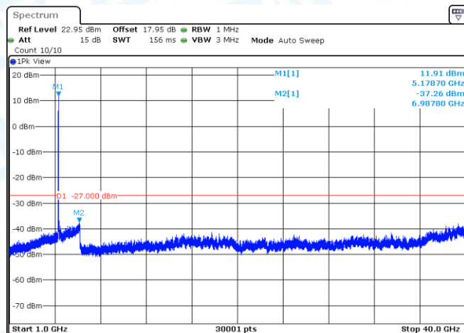
11AX20SISO-Ant1-5180-1000~40000-PASS
