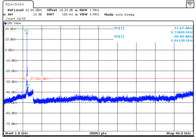
11AC20SISO-Ant1-5745-1000~40000-PASS
