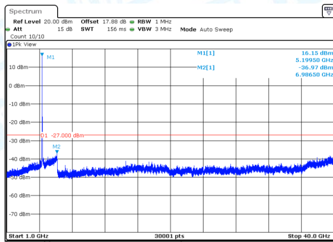
11AX20SISO-Ant1-5180-1000~40000-PASS
