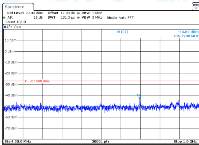
11AX20SISO-Ant1-5180-30~1000-PASS
