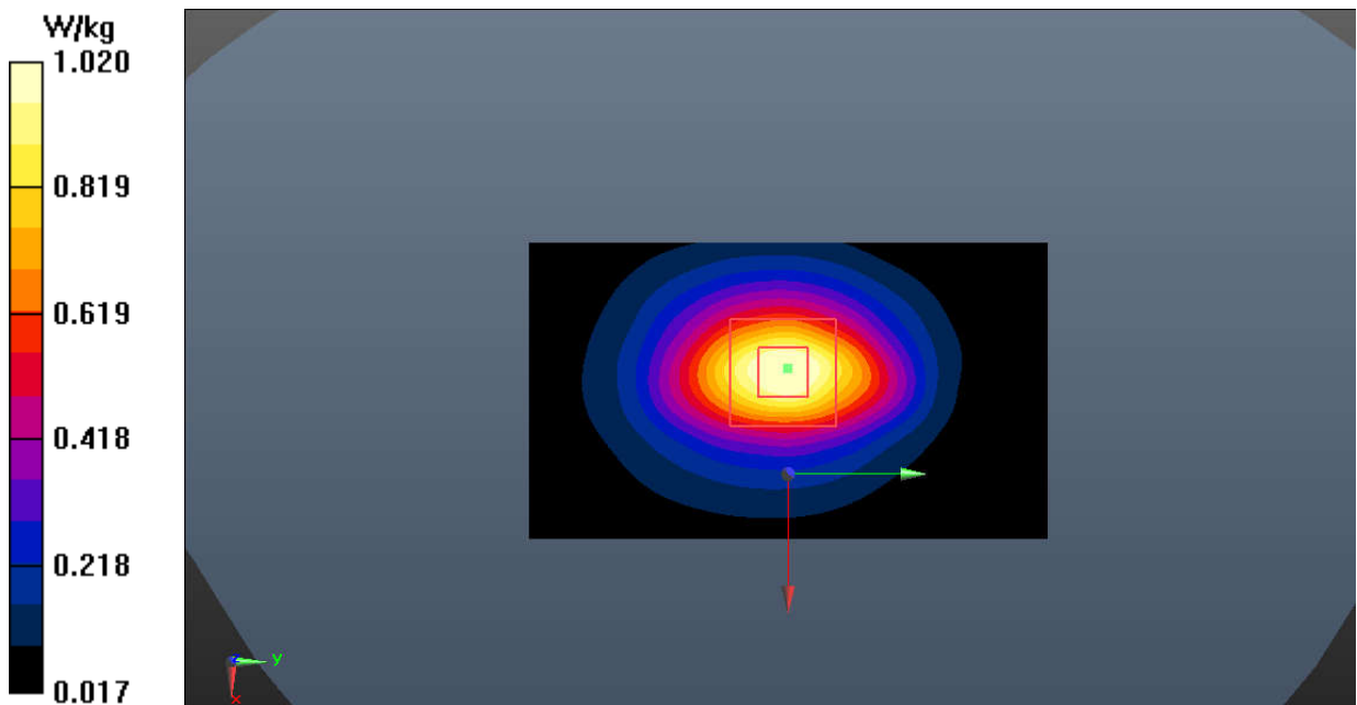
Fig.4 GSM1900 Body
