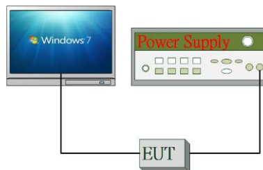
Fig. 2-3 Conduction Configuration
