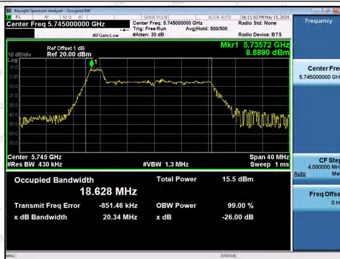
11AX20SISO-Ant1-5745-26Tone-RU0
