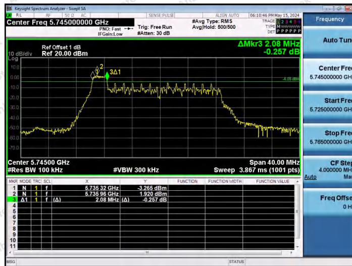
11AX20SISO-Ant1-5745-26Tone-RU0-PASS
