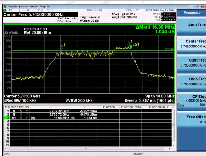
11AX20SISO-Ant1-5745-52Tone-RU40-PASS
