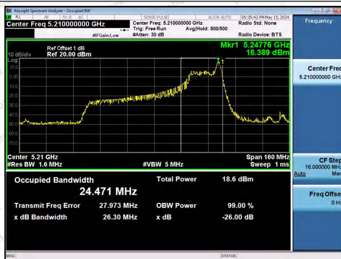
11AX80SISO-Ant1-5210-26Tone-RU36
