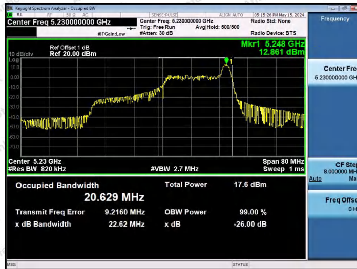
11AX40SISO-Ant1-5230-26Tone-RU17
