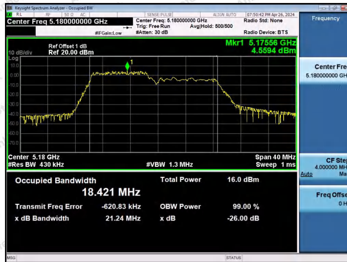
11AX20SISO-Ant1-5180-106Tone-RU53
