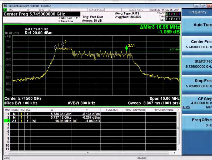
11AX20SISO-Ant1-5745-52Tone-RU37-PASS
