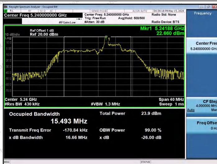
11AX20SISO-Ant1-5240-52Tone-RU39
