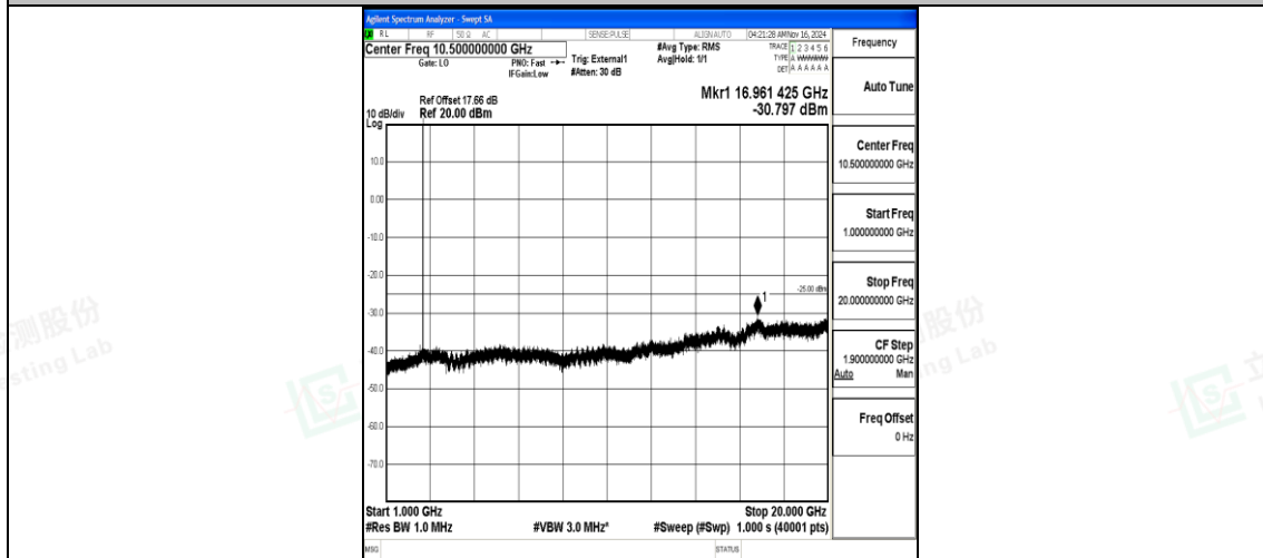
Band41_10MHz_16QAM_40620_1RB#0_1000~20000_1000~20000
