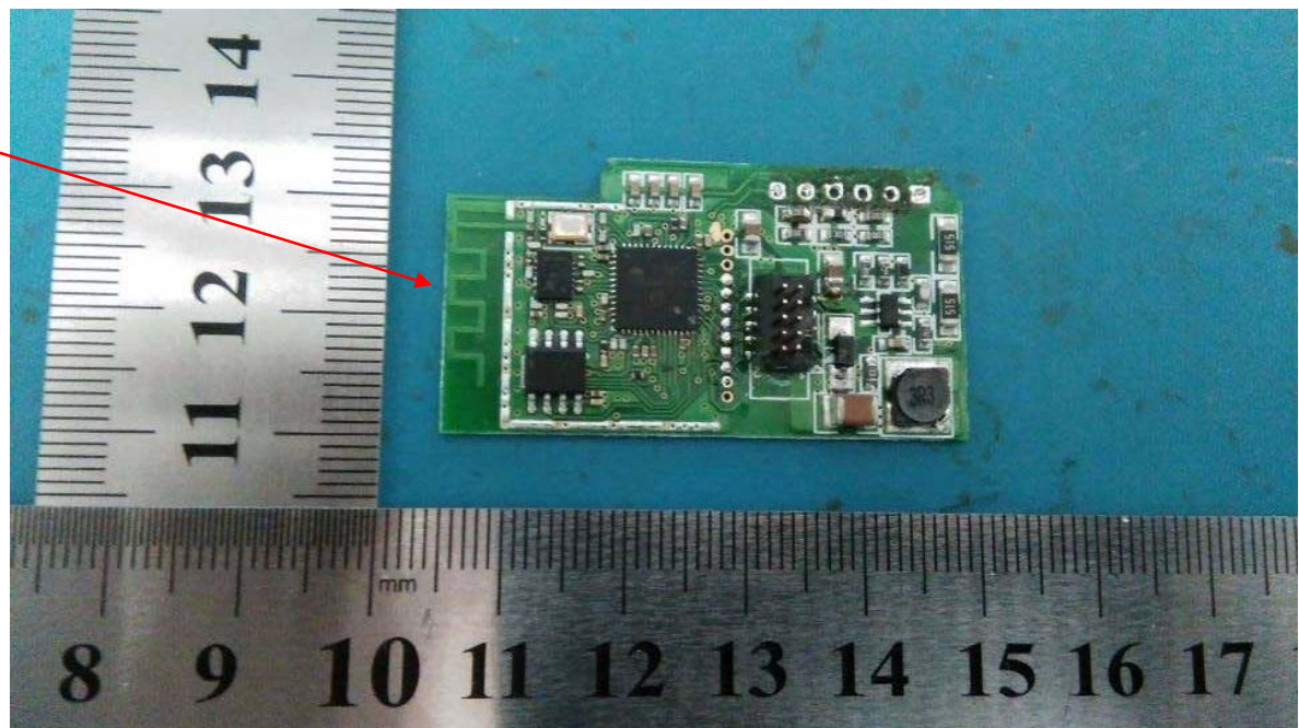
EUT- RF Module Top View
