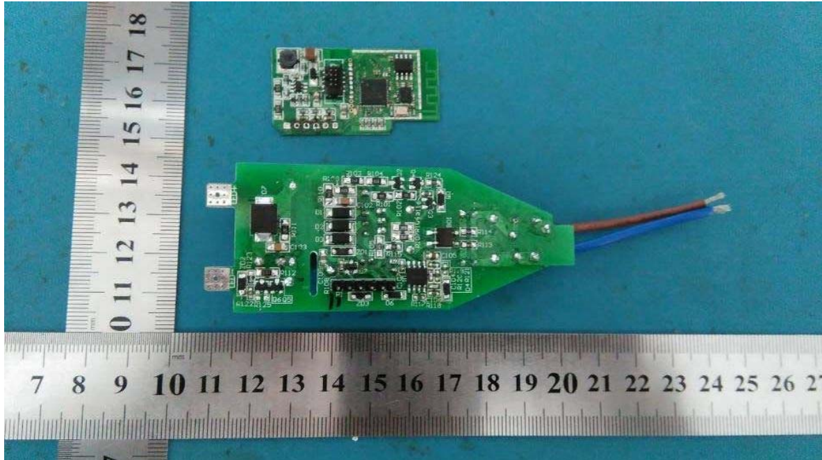
EUT- PCB Board Uncover View
