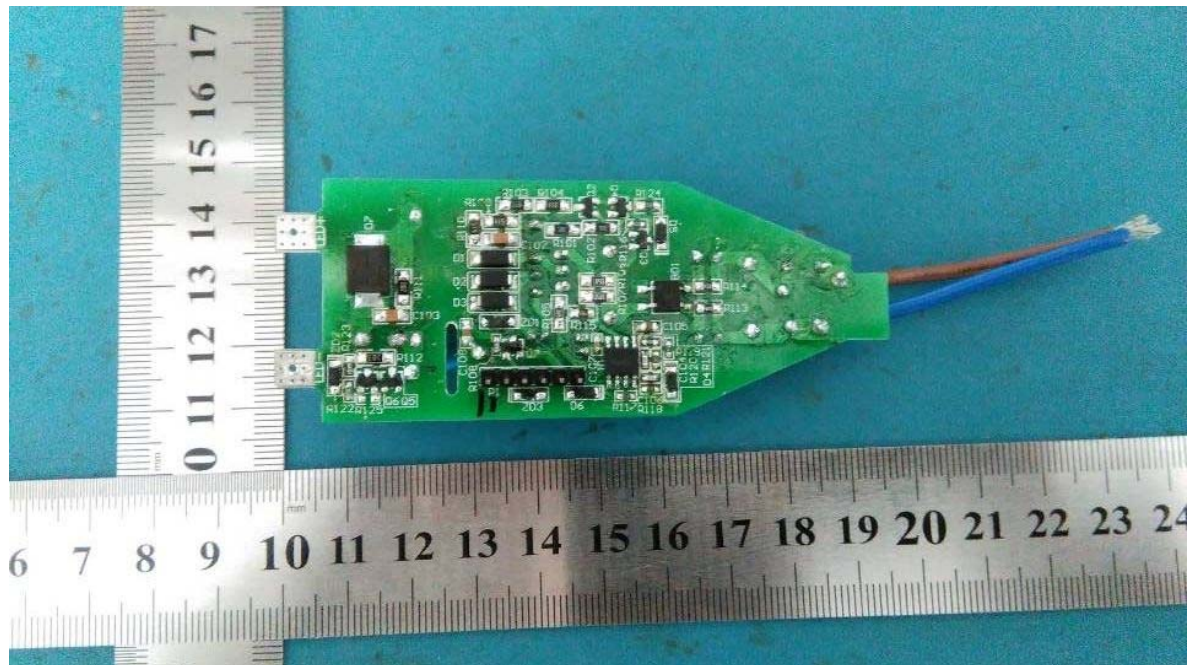
EUT- Power Board Bottom View
