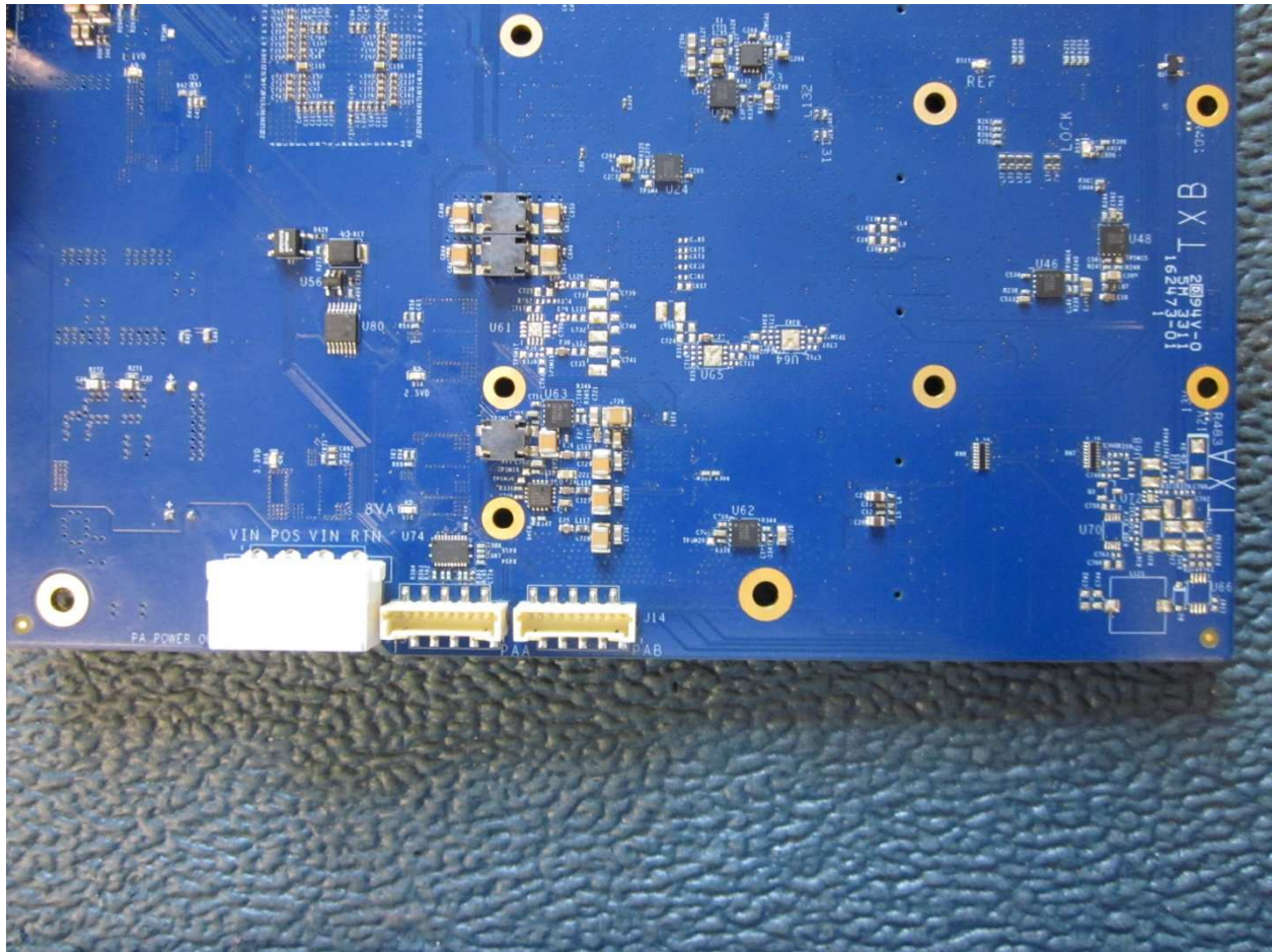
Motherboard – Back #2
