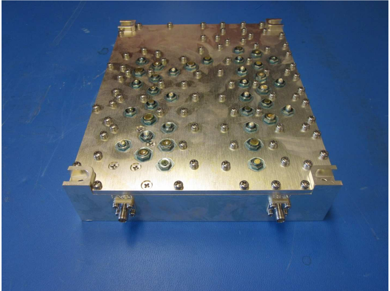
Duplexer #1
