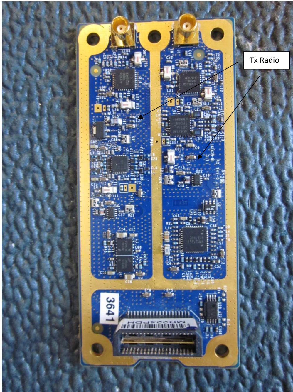
Tx Board – Front
