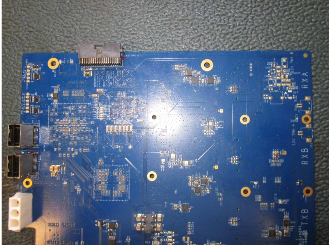
Motherboard – Back #3
