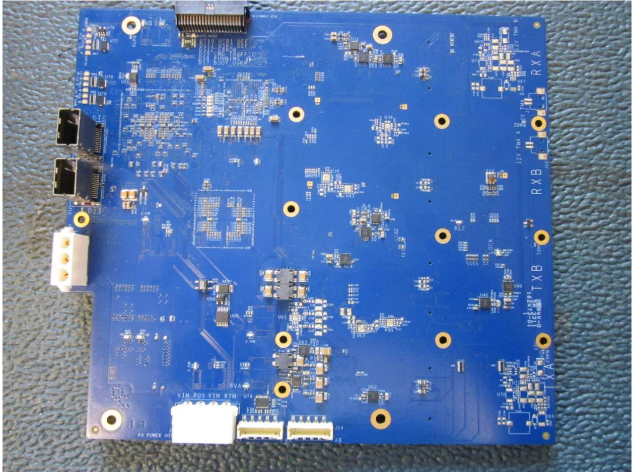
Motherboard – Back #1
