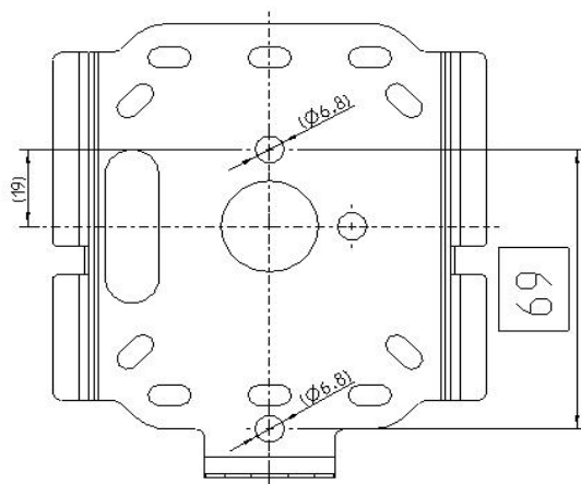
FIGURE 1-6: Figure 4 - Metal Bracket for imagotag AP-2010
