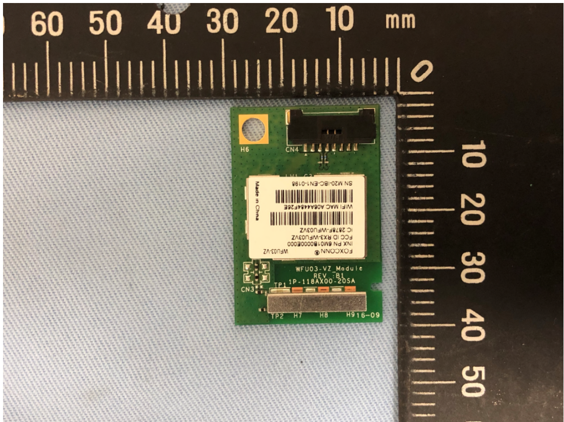
Modified sample for additional solder pad of shield house(reference only)
