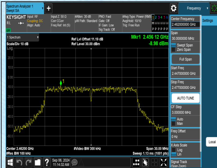
11N20MIMO-Ant3-2462-0~Reference-PASS
