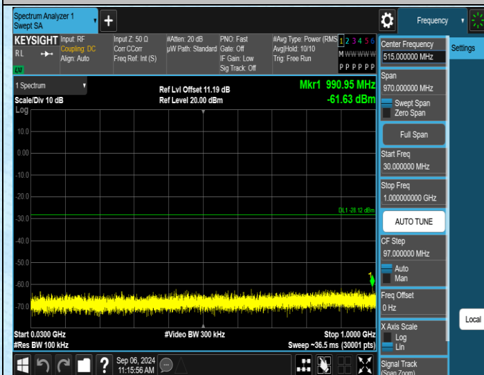
11N20MIMO-Ant4-2462-30~1000-PASS
