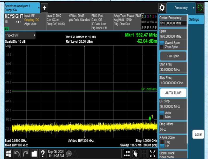
11N20MIMO-Ant3-2462-30~1000-PASS
