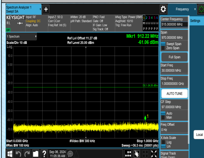
11N20SISO-Ant4-2437-30~1000-PASS
