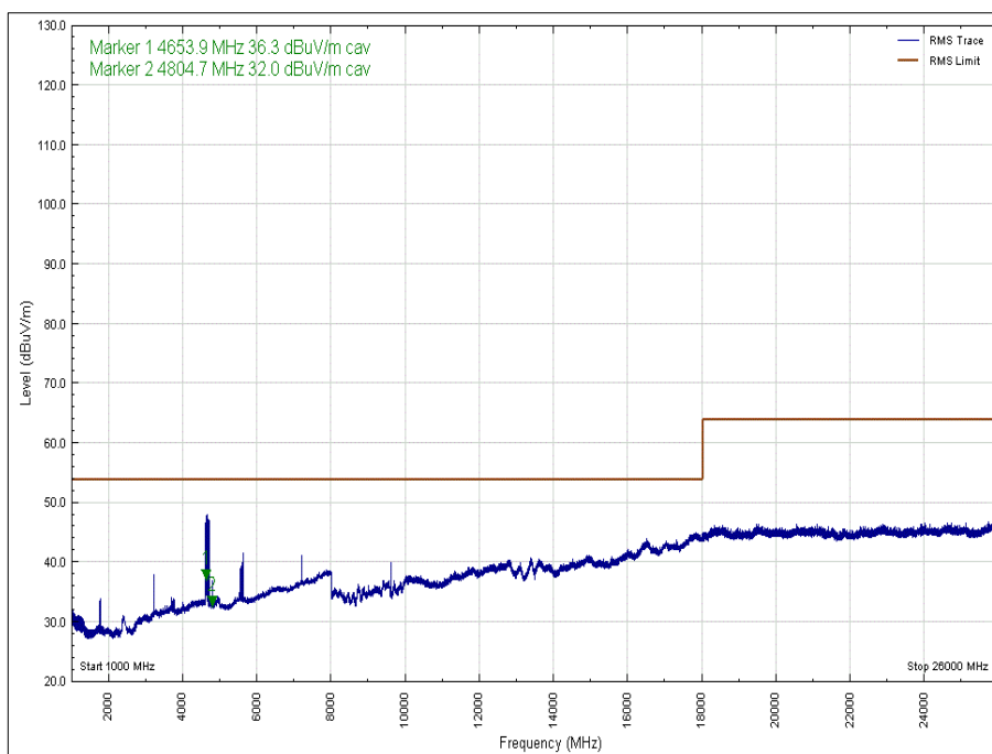
Figure 32 - 2402 MHz - 1 GHz to 26 GHz, Polarity: Vertical, EUT Orientation: Y, Average
