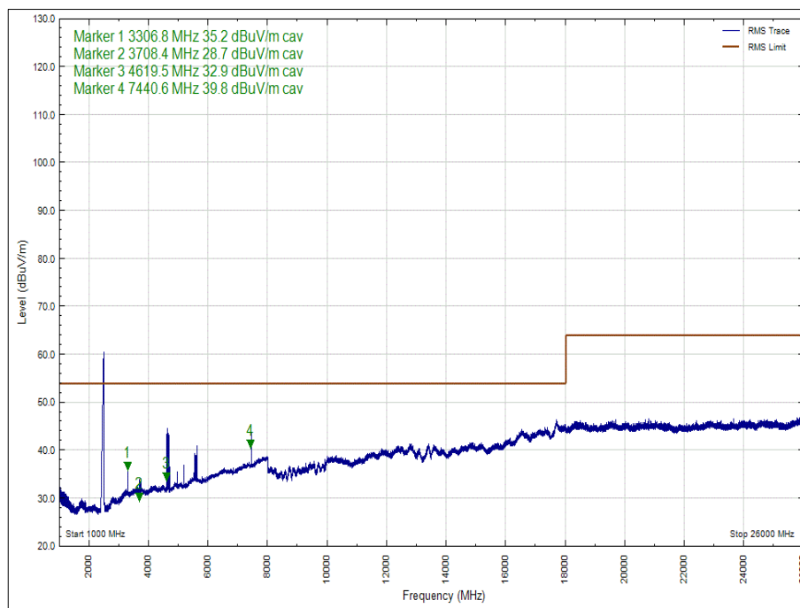
Figure 69 - 2480 MHz - 1 GHz to 26 GHz, Polarity: Horizontal, EUT Orientation: Y, Average
