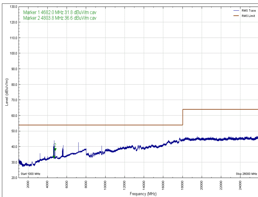
Figure 33 - 2402 MHz - 1 GHz to 26 GHz, Polarity: Horizontal, EUT Orientation: Y, Average
