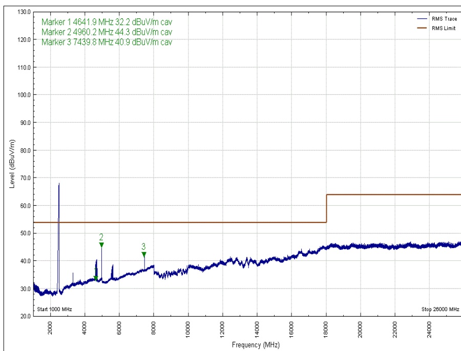
Figure 64 - 2480 MHz - 1 GHz to 26 GHz, Polarity: Vertical, EUT Orientation: X, Average
