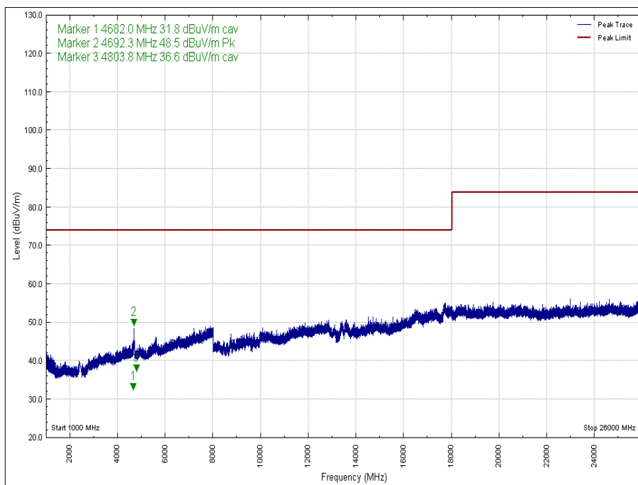
Figure 31 - 2402 MHz - 1 GHz to 26 GHz, Polarity: Horizontal, EUT Orientation: Y, Peak
