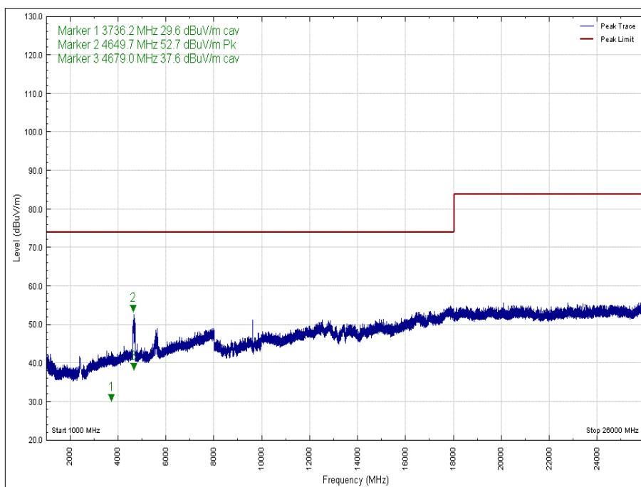
Figure 34 - 2402 MHz - 1 GHz to 26 GHz, Polarity: Vertical, EUT Orientation: Z, Peak
