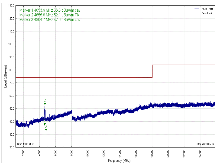
Figure 30 - 2402 MHz - 1 GHz to 26 GHz, Polarity: Vertical, EUT Orientation: Y, Peak
