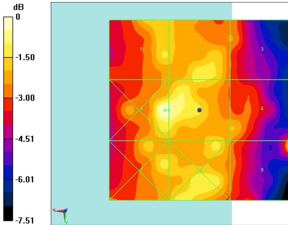
Fig B.3 HAC RF E-Field CDMA BC0 Middle
