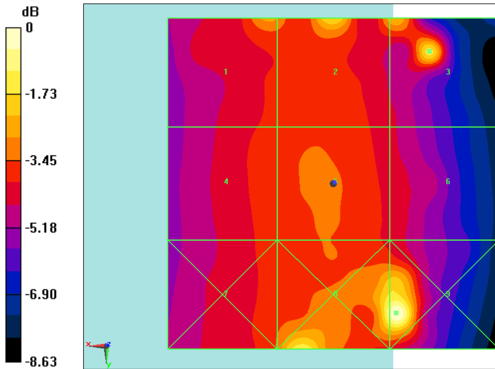
Fig B.5 HAC RF E-Field CDMA BC10 Low
