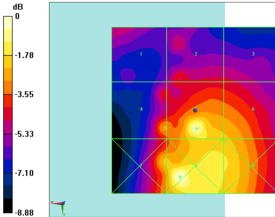
Fig B.4 HAC RF E-Field CDMA BC1 Middle
