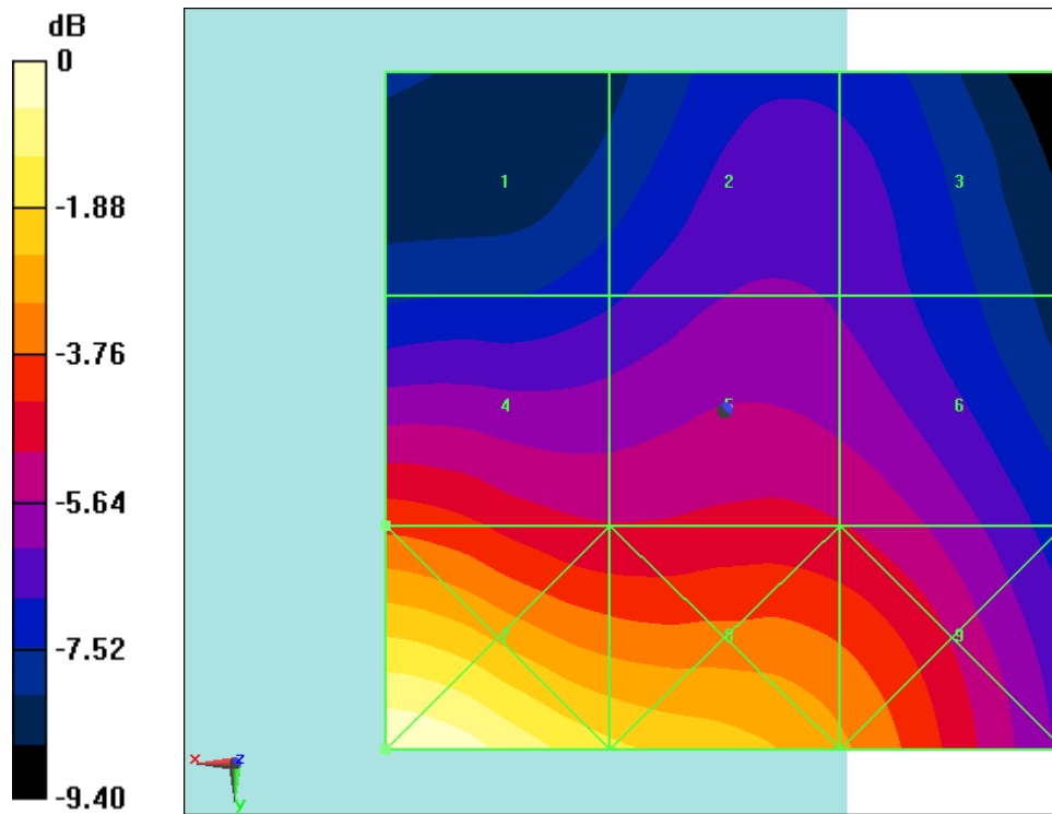
Fig B.8 HAC RF E-Field WiFi2.4G 11b
