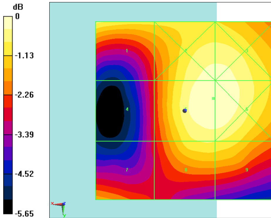
Fig B.7 HAC RF E-Field LTE Band41 Power Class 3 QPSK CH39750
