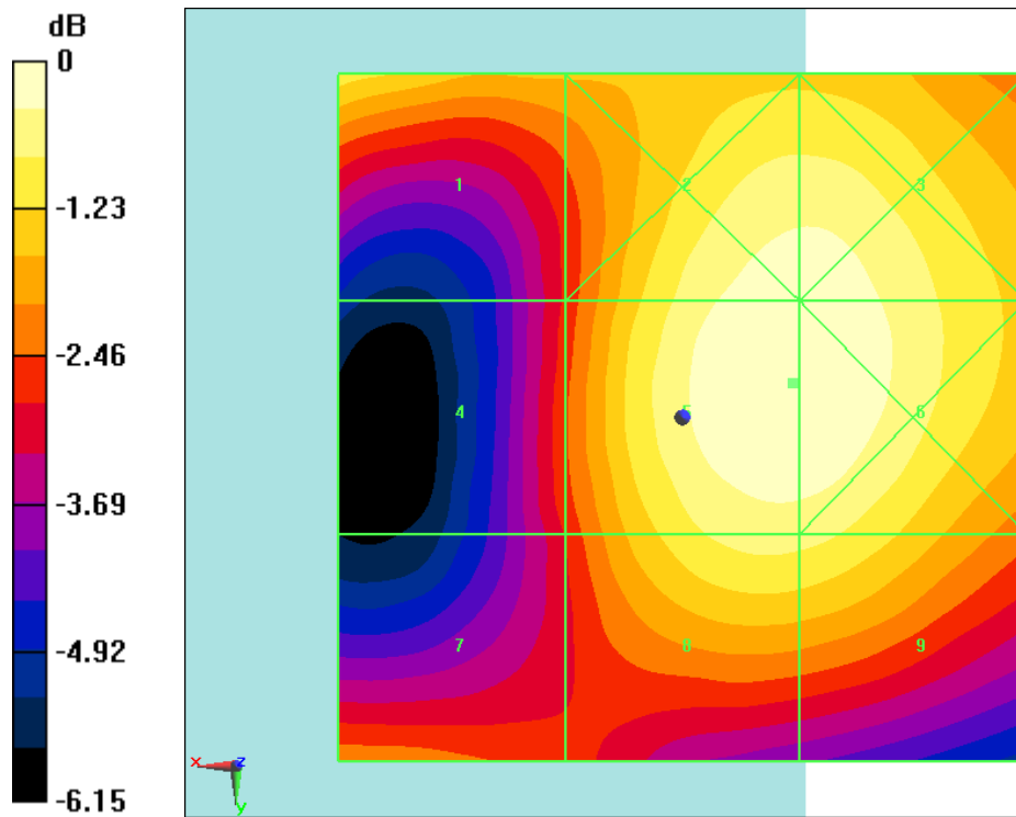
Fig B.6 HAC RF E-Field LTE Band41 Power Class 2 QPSK CH39750
