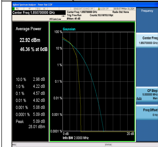
Band2-1.4MHz-16QAM-18607-1RB#0-PASS
