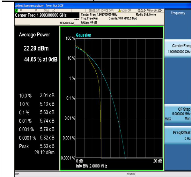
Band2-1.4MHz-16QAM-19193-1RB#0-PASS
