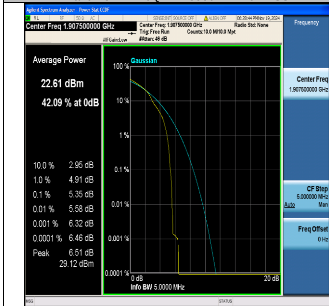
Band2-5MHz-16QAM-19175-1RB#0-PASS
