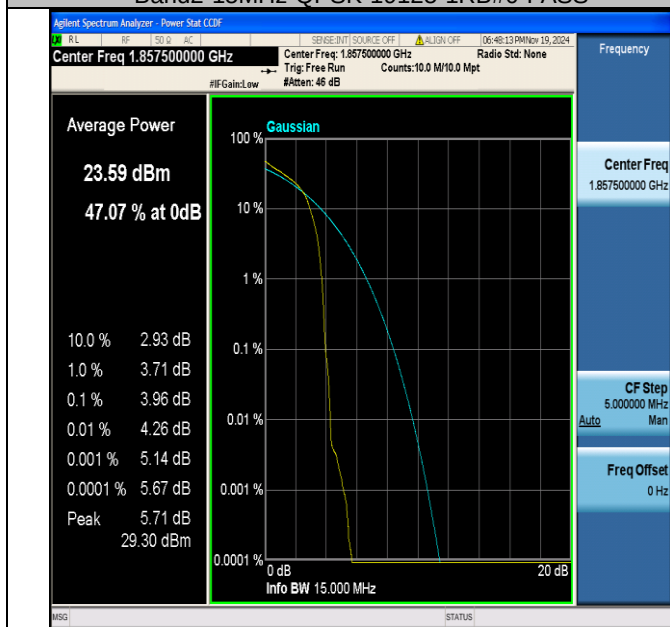
Band2-15MHz-16QAM-18675-1RB#0-PASS
