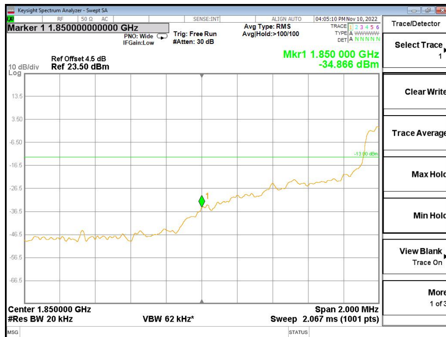
Band2-Low Channel-15MHz Bandwidth-6RB-QPSK
