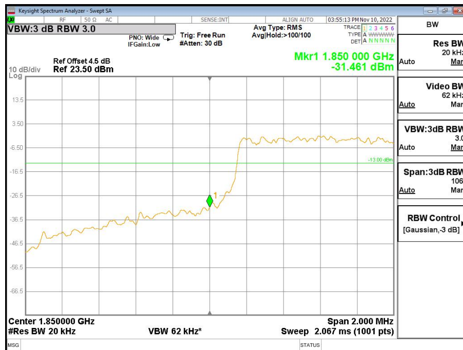
Band2-Low Channel-1.4MHz Bandwidth-6RB-QPSK
