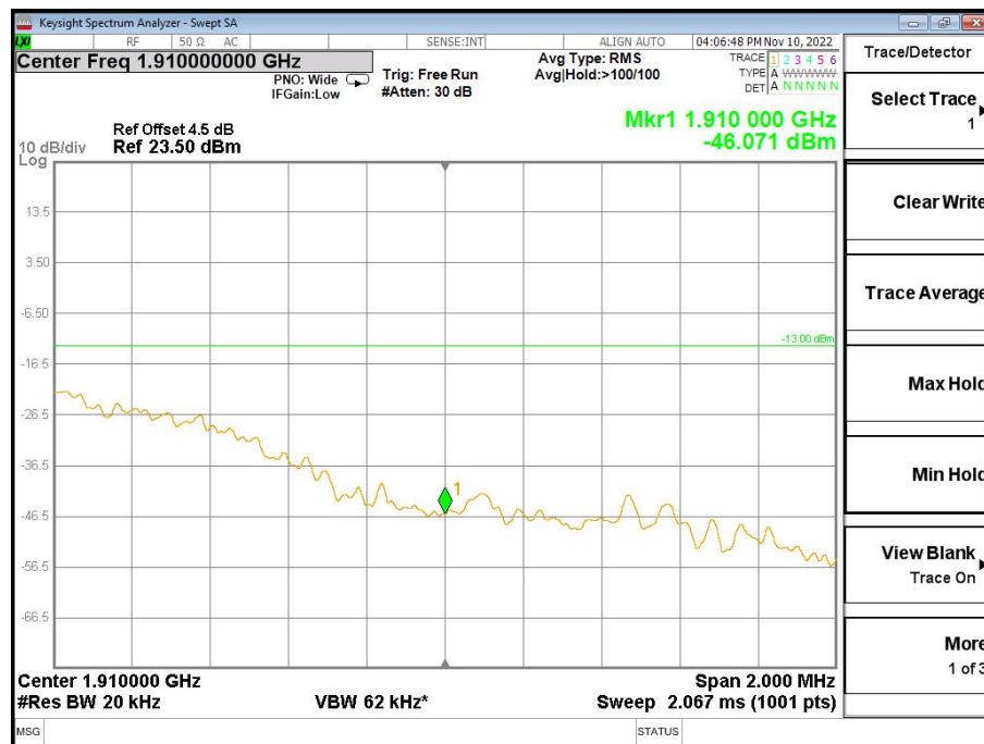
Band2-High Channel-20MHz Bandwidth-6RB-QPSK
