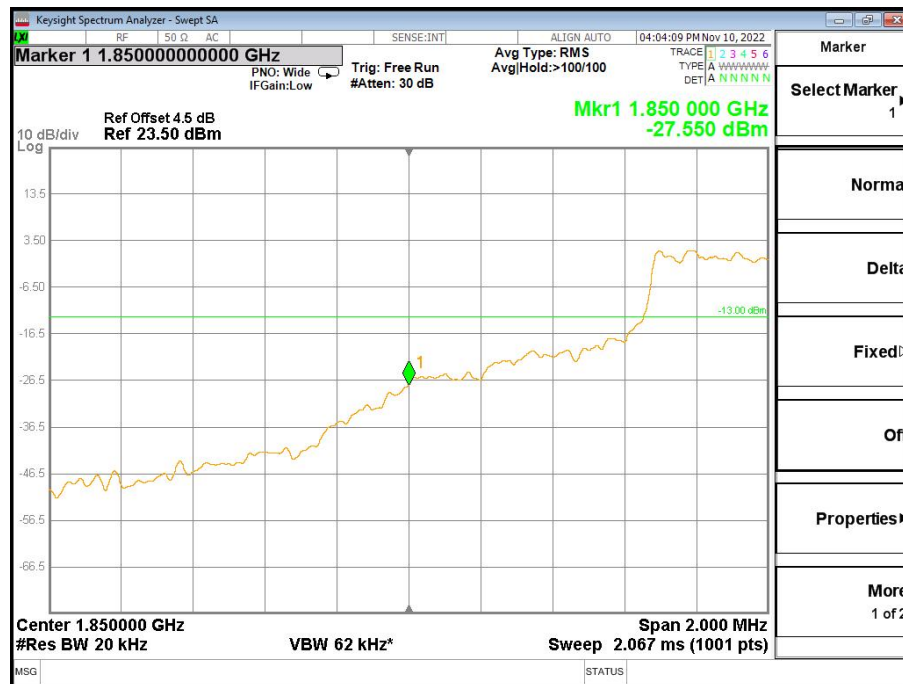
Band2-Low Channel-10MHz Bandwidth-5RB-16QAM
