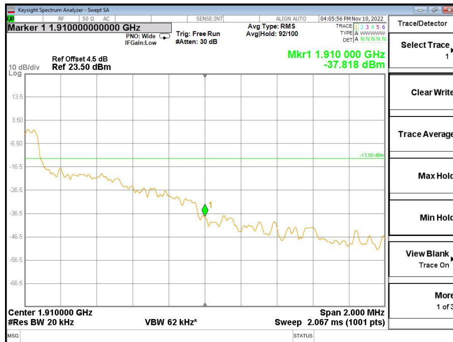
Band2-High Channel-15MHz Bandwidth-5RB-16QAM
