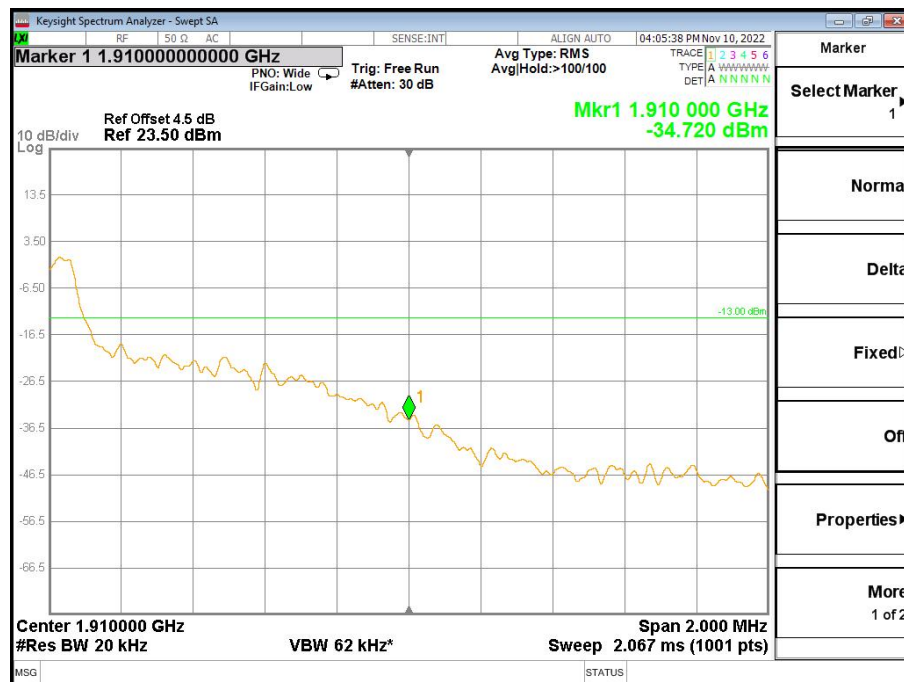
Band2-High Channel-15MHz Bandwidth-6RB-QPSK
