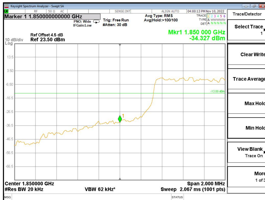
Band2-Low Channel-3MHz Bandwidth-6RB-QPSK
