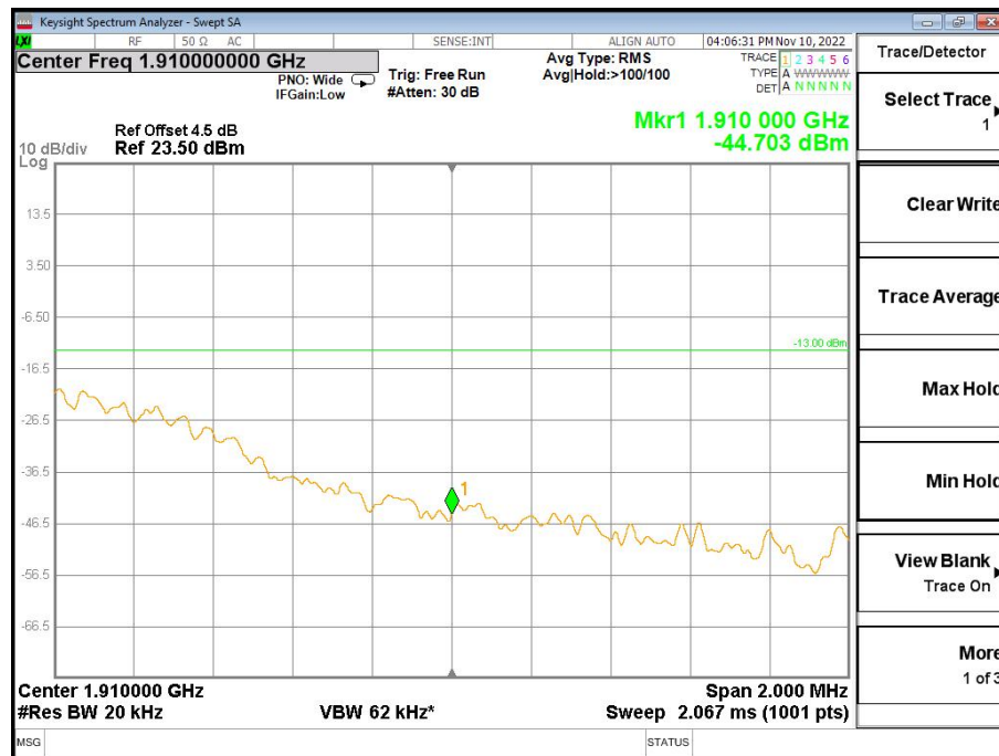
Band2-High Channel-20MHz Bandwidth-5RB-16QAM
