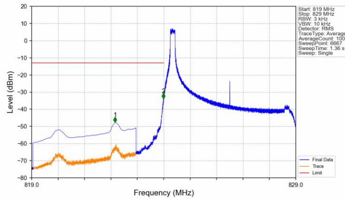
Band26b_5MHz_QPSK_LCH_826.5MHz_RB_1_0_NTNV
