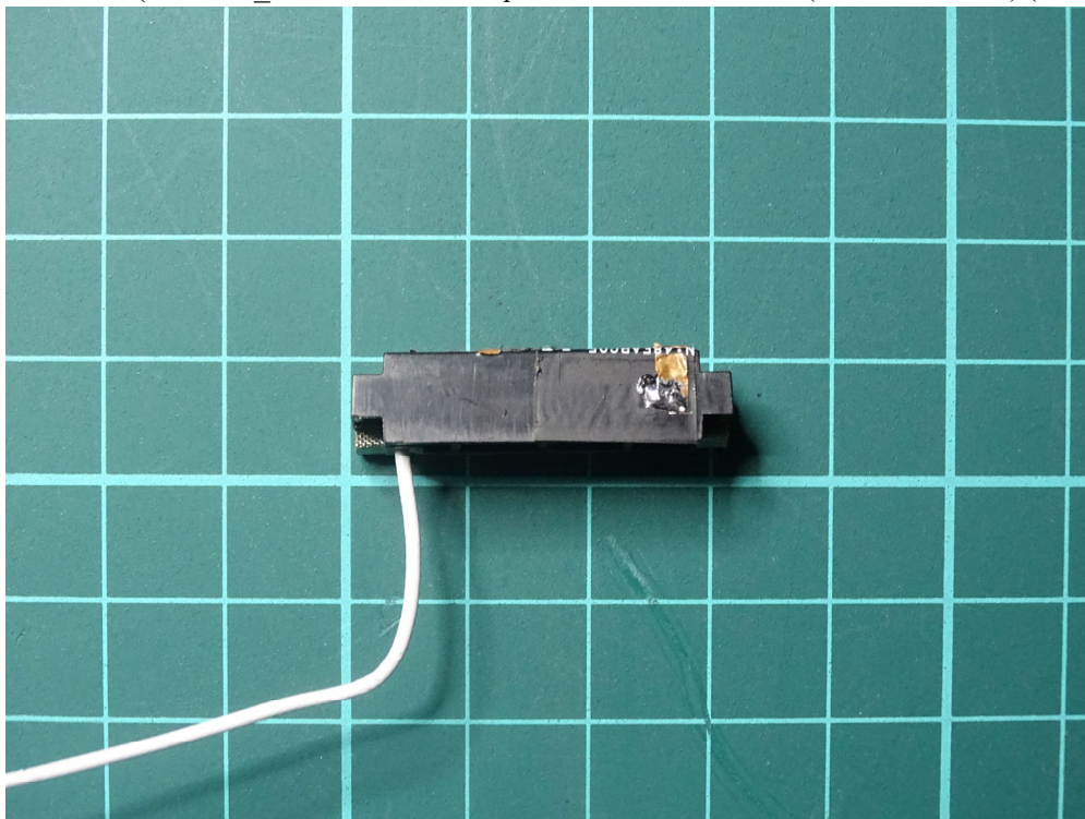
(62) EUT Photo (Antenna_Wistron Neweb Corporation / DC33002IK0L (81EABG15.G09) (Main))
