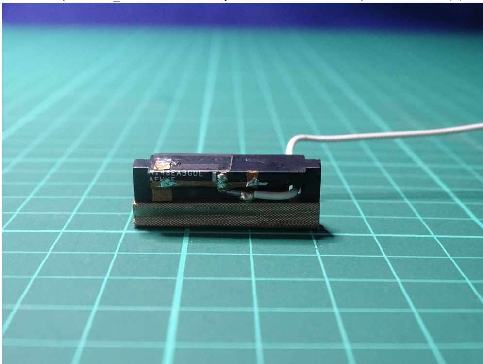
(63) EUT Photo (Antenna_Wistron Neweb Corporation / DC33002IK0L (81EABG15.G09) (Main))
