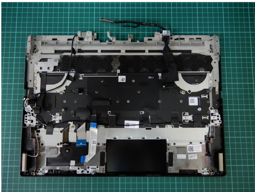
(55) EUT Photo
