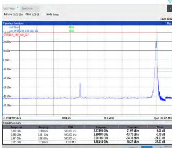
1-N77-3700-3980--30-100-H-5-CP-QPSK-Edge_1RB_Right-1@272-Ant1-PASS-see graph
