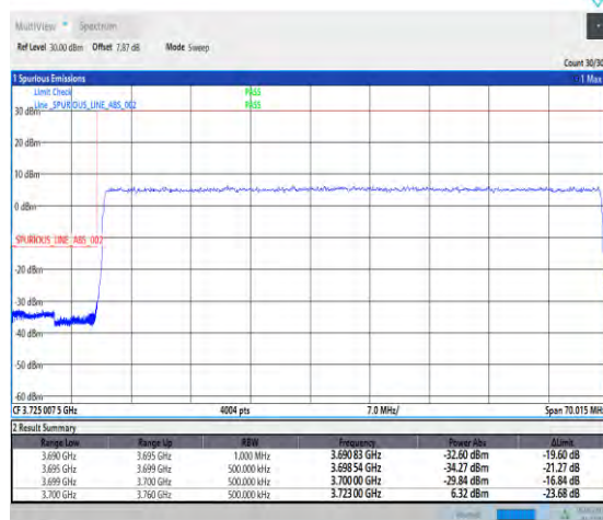
1-N77-3700-3980--30-60-L-3-DFT-PI2BPSK-Outer_Full-162@0-Ant1-PASS-see graph
