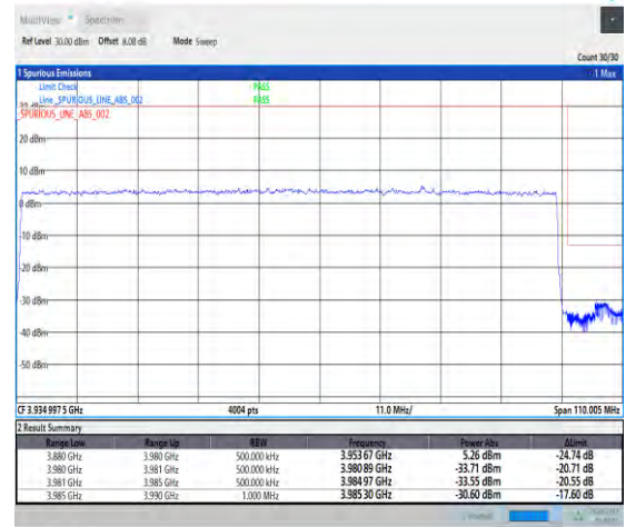
1-N77-3700-3980--30-100-H-3-DFT-PI2BPSK-Out er_Full-270@0-Ant1-PASS-see graph
