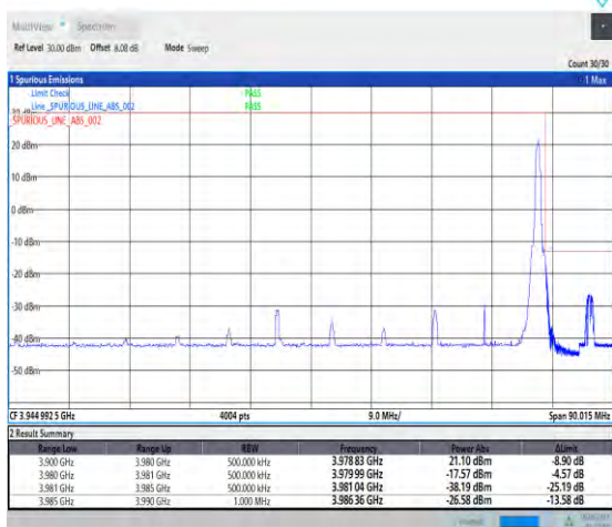
1-N77-3700-3980--30-80-H-2-DFT-PI2BPSK-Edge_1R_B_Right-1@216-Ant1-PASS-see graph
