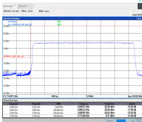
1-N77-3700-3980--30-40-L-3-DFT-PI2BPSK-Outer_Full-100@0-Ant1-PASS-see graph
