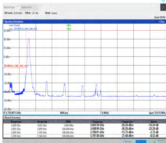
1-N77-3700-3980--30-60-L-1-DFT-PI2BPSK-Edge_1R_B_Left-1@0-Ant1-PASS-see graph
