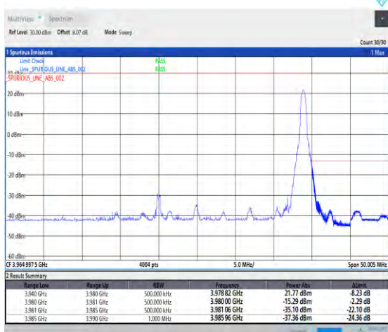
1-N77-3700-3980--30-40-H-5-CP-QPSK-Edge_1RB_Right-1@105-Ant1-PASS-see graph
