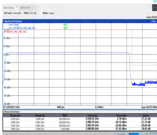
1-N77-3700-3980--30-50-H-6-CP-QPSK-Outer_Fu ll-133@0-Ant1-PASS-see graph
