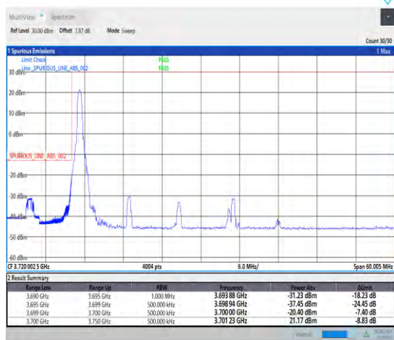
1-N77-3700-3980--30-50-L-1-DFT-PI2BPSK-Edge_1R_B_Left-1@0-Ant1-PASS-see graph
