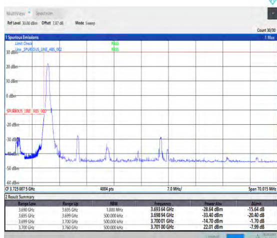
1-N77-3700-3980--30-60-L-4-CP-QPSK-Edge_1RB_L eft-1@0-Ant1-PASS-see graph
