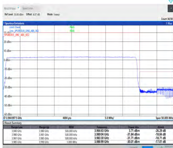
1-N77-3700-3980--30-40-H-6-CP-QPSK-Outer_Full-106@0-Ant1-PASS-see graph
