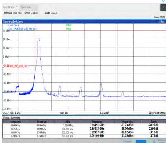
1-N77-3700-3980--30-40-L-1-DFT-PI2BPSK-Edge_1R_B_Left-1@0-Ant1-PASS-see graph
