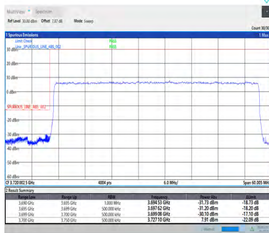
1-N77-3700-3980--30-50-L-3-DFT-PI2BPSK-Outer_Full-128@0-Ant1-PASS-see graph
