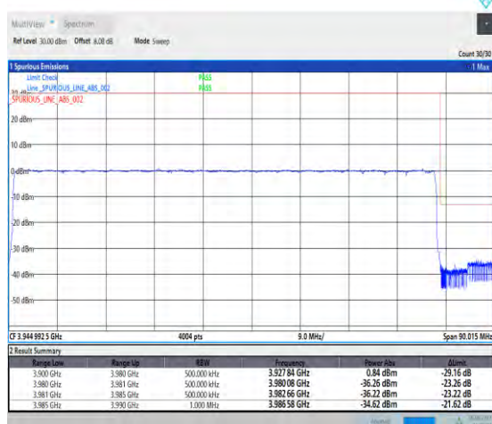
1-N77-3700-3980--30-80-H-6-CP-QPSK-Outer_Full-217@0-Ant1-PASS-see graph
