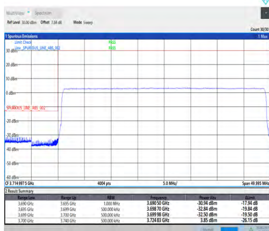
1-N77-3700-3980--30-40-L-6-CP-QPSK-Outer_Ful I-106@0-Ant1-PASS-see graph
