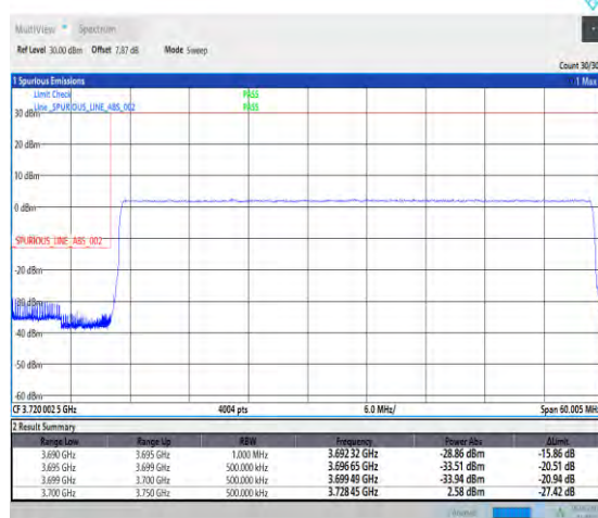
1-N77-3700-3980--30-50-L-6-CP-QPSK-Outer_Ful I-133@0-Ant1-PASS-see graph
