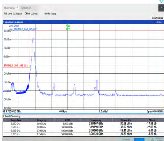
1-N77-3700-3980--30-50-L-4-CP-QPSK-Edge_1RB_L eft-1@0-Ant1-PASS-see graph
