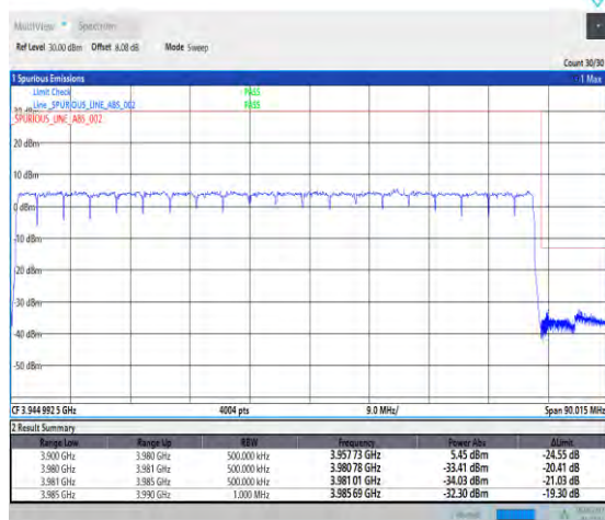
1-N77-3700-3980--30-80-H-3-DFT-PI2BPSK-Outer_Full-216@0-Ant1-PASS-see graph
