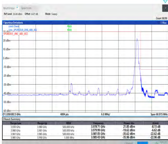
1-N77-3700-3980--30-50-H-5-CP-QPSK-Edge_1RB_R ight-1@132-Ant1-PASS-see graph
