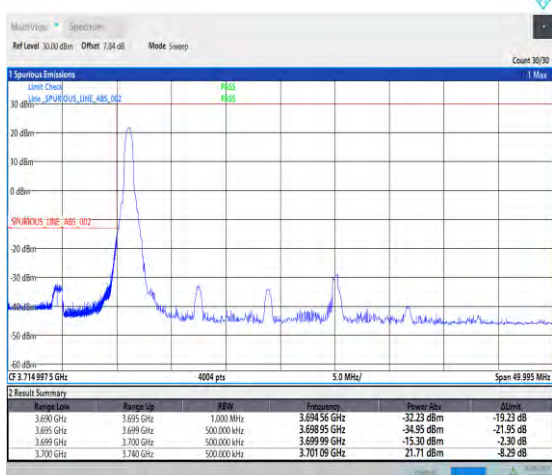
1-N77-3700-3980--30-40-L-4-CP-QPSK-Edge_1RB_L eft-1@0-Ant1-PASS-see graph
