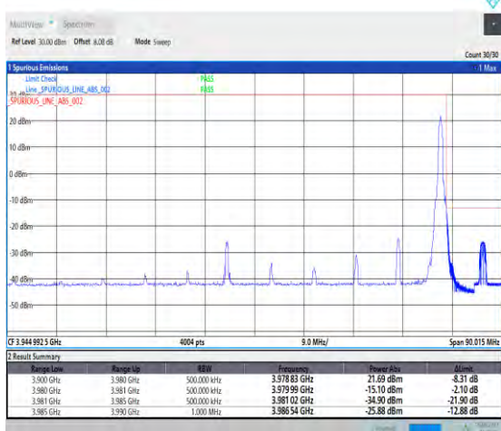
1-N77-3700-3980--30-80-H-5-CP-QPSK-Edge_1RB_Right-1@216-Ant1-PASS-see graph
