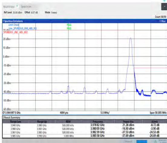
1-N77-3700-3980--30-40-H-2-DFT-PI2BPSK-Edge_1R_B_Right-1@105-Ant1-PASS-see graph
