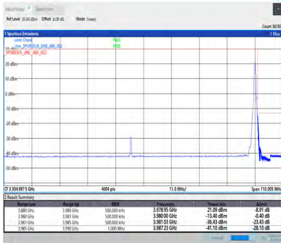
1-N77-3700-3980--30-100-H-2-DFT-PI2BPSK-Edge_1 RB_Right-1@272-Ant1-PASS-see graph
