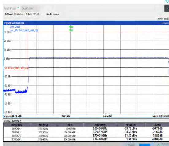
1-N77-3700-3980--30-60-L-6-CP-QPSK-Outer_Ful I-162@0-Ant1-PASS-see graph
