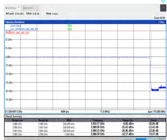
1-N77-3700-3980--30-100-H-6-CP-QPSK-Outer_F ull-273@0-Ant1-PASS-see graph
