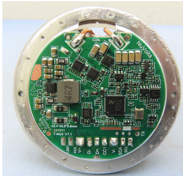
Qi2 MPP/BPP Coil and PCBA (127.7kHz, 360kHz)
