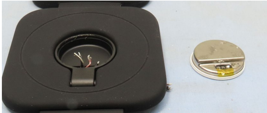
Apple Watch Coil and PCBA (326.5kHz / 1.778MHz)
