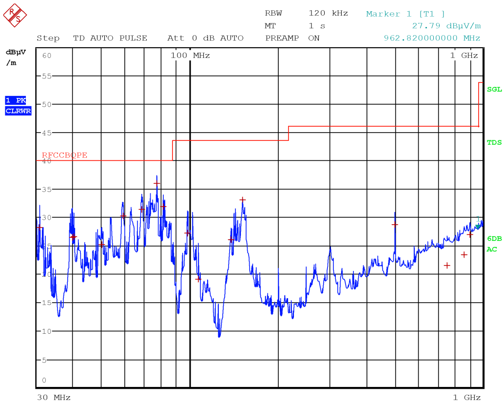
GSM 1880 MHz and wifi 802.11a Multiple Chain 5300 MHz, vertical polarization
