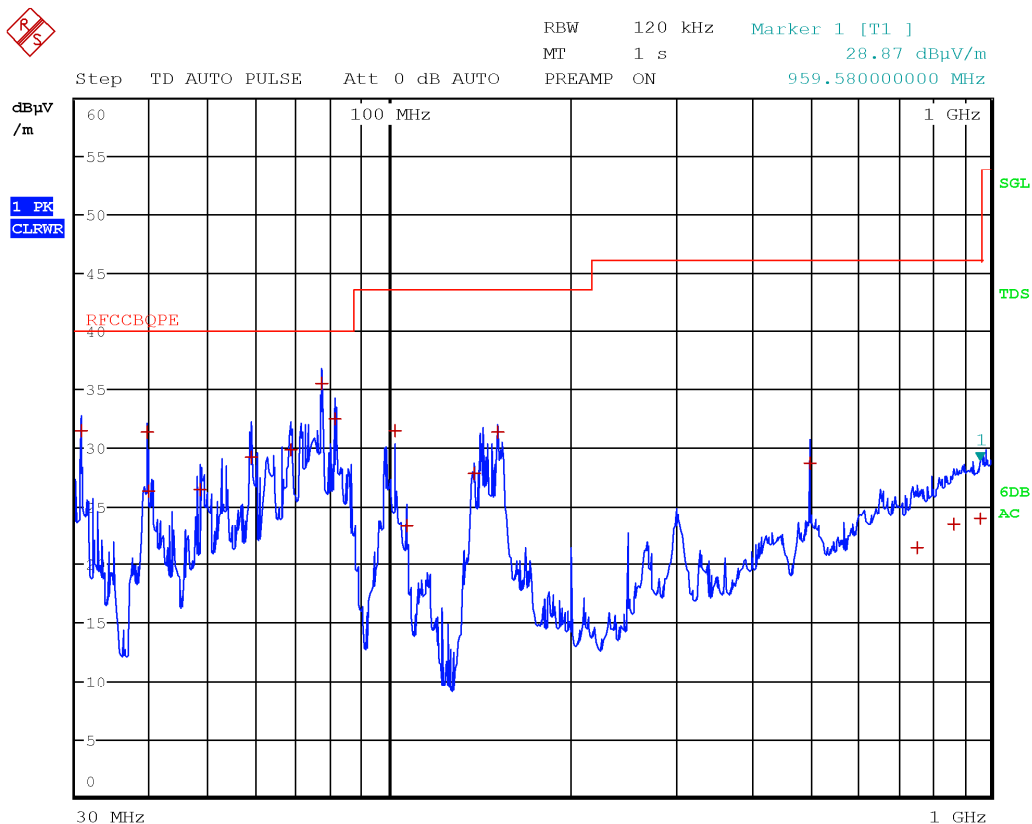
LTE B41 (5MHz) 2593 MHz and wifi 802.11a 6Mbps Multiple Chain 5300 MHz, vertical polarization
