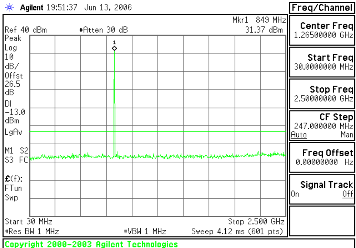
Figure 7-5: Out of Band emission at antenna terminals – GSM CH High
