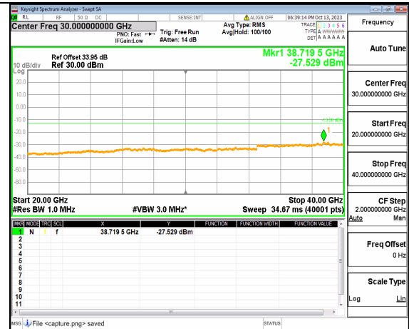
5A_n77(3700-3980MHz) (20GHz-40GHz) 100M DFT-s-OFDM BPSK Edge_1RB_Left High
