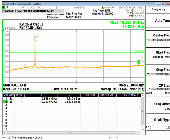
5A_n77(3700-3980MHz) (30MHz-20GHz) 90M DFT-s-OFDM BPSK Outer_Full Mid
