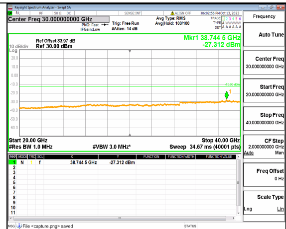
5A_n77(3700-3980MHz) (20GHz-40GHz) 90M DFT-s-OFDM QPSK Edge_1RB_Left Low
