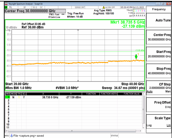
5A_n77(3700-3980MHz) (20GHz-40GHz) 70M DFT-s-OFDM QPSK Edge_1RB_Left High
