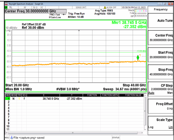
5A_n77(3700-3980MHz) (20GHz-40GHz) 90M DFT-s-OFDM BPSK Edge_1RB_Left Low
