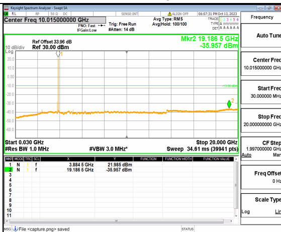
5A_n77(3700-3980MHz) (30MHz-20GHz) 90M DFT-s-OFDM BPSK Edge_1RB_Right Mid
