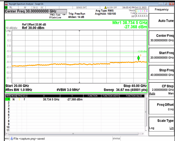
5A_n77(3700-3980MHz) (20GHz-40GHz) 90M DFT-s-OFDM BPSK Outer_Full Mid
