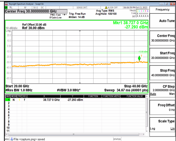
5A_n77(3700-3980MHz) (20GHz-40GHz) 90M DFT-s-OFDM BPSK Edge_1RB_Left Mid
