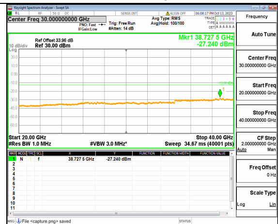
5A_n77(3700-3980MHz) (20GHz-40GHz) 90M DFT-s-OFDM BPSK Edge_1RB_Right Mid
