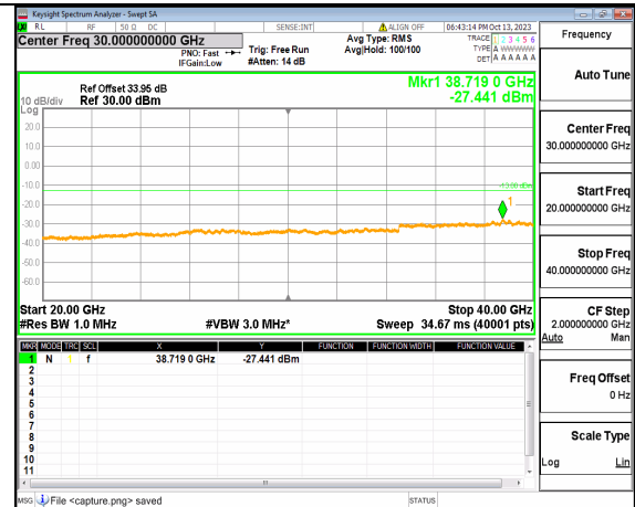
5A_n77(3700-3980MHz) (20GHz-40GHz) 100M DFT-s-OFDM QPSK Edge_1RB_Left High
