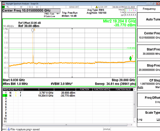
5A_n77(3700-3980MHz) (30MHz-20GHz) 90M DFT-s-OFDM BPSK Edge_1RB_Left Mid
