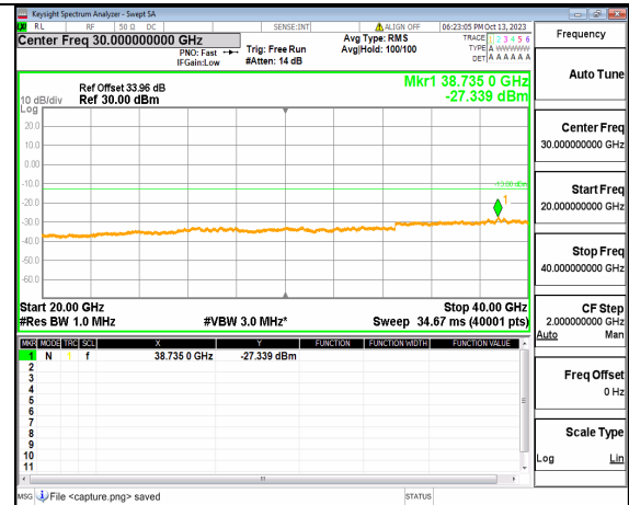
5A_n77(3700-3980MHz) (20GHz-40GHz) 100M DFT-s-OFDM BPSK Edge_1RB_Left Low
