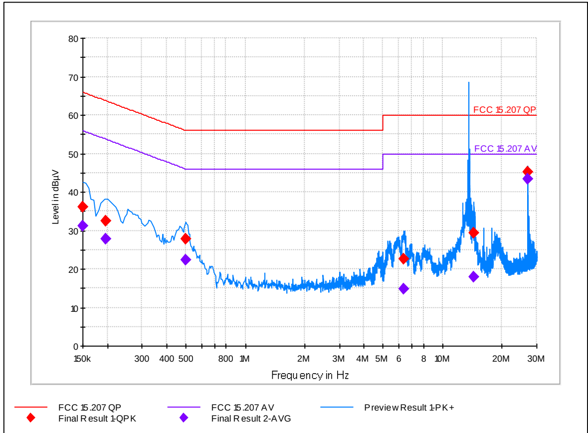
Figure 39. AC Conducted emission.
