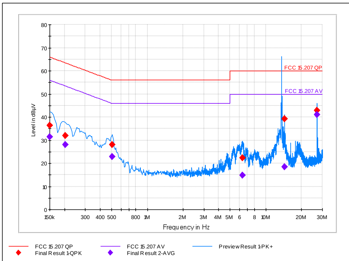
Figure 33. AC Conducted emission.
