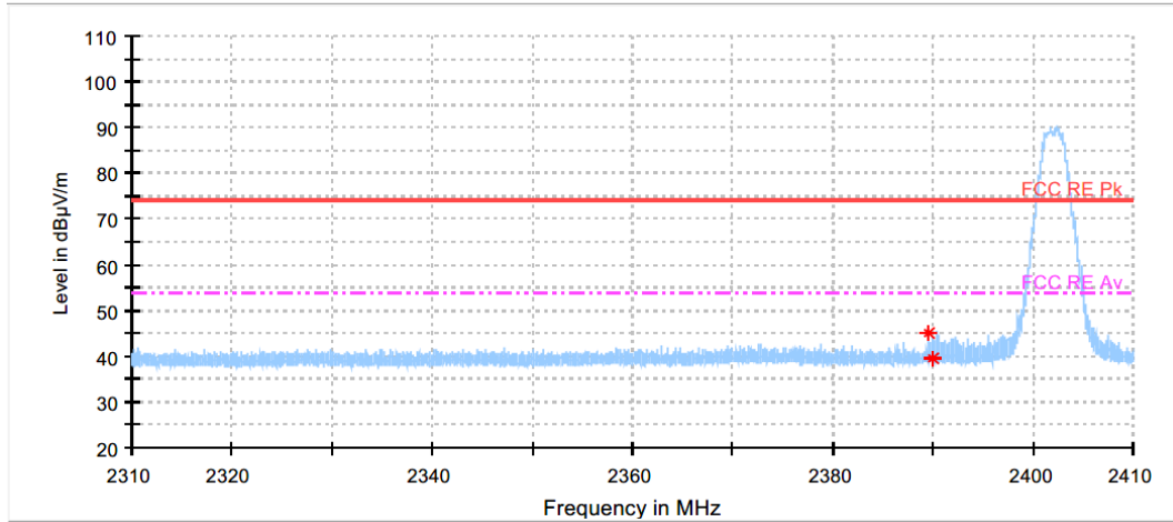
BLE 2Mbps, Lowest Channel (2 402 MHz)_Peak
