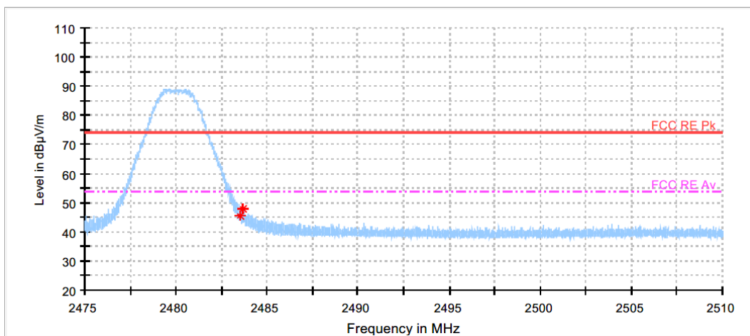
BLE 2Mbps, Highest Channel (2 480 MHz)_Peak
