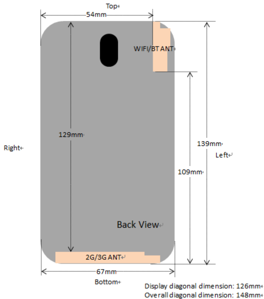
Fig.14.1 EUT Antenna Locations
