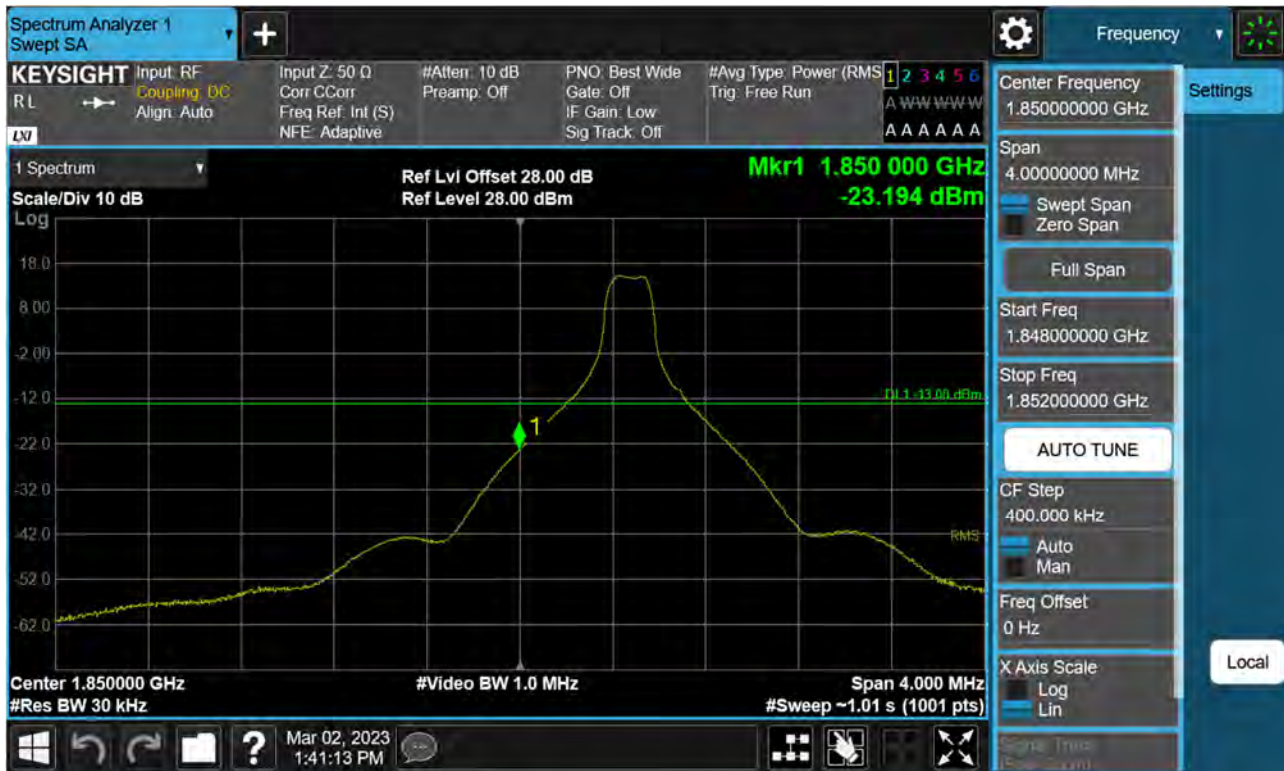
Sub6 n2. Lower Band Edge Plot (15 M BW Ch.371500 BPSK_RB1_Offset 0) -1
