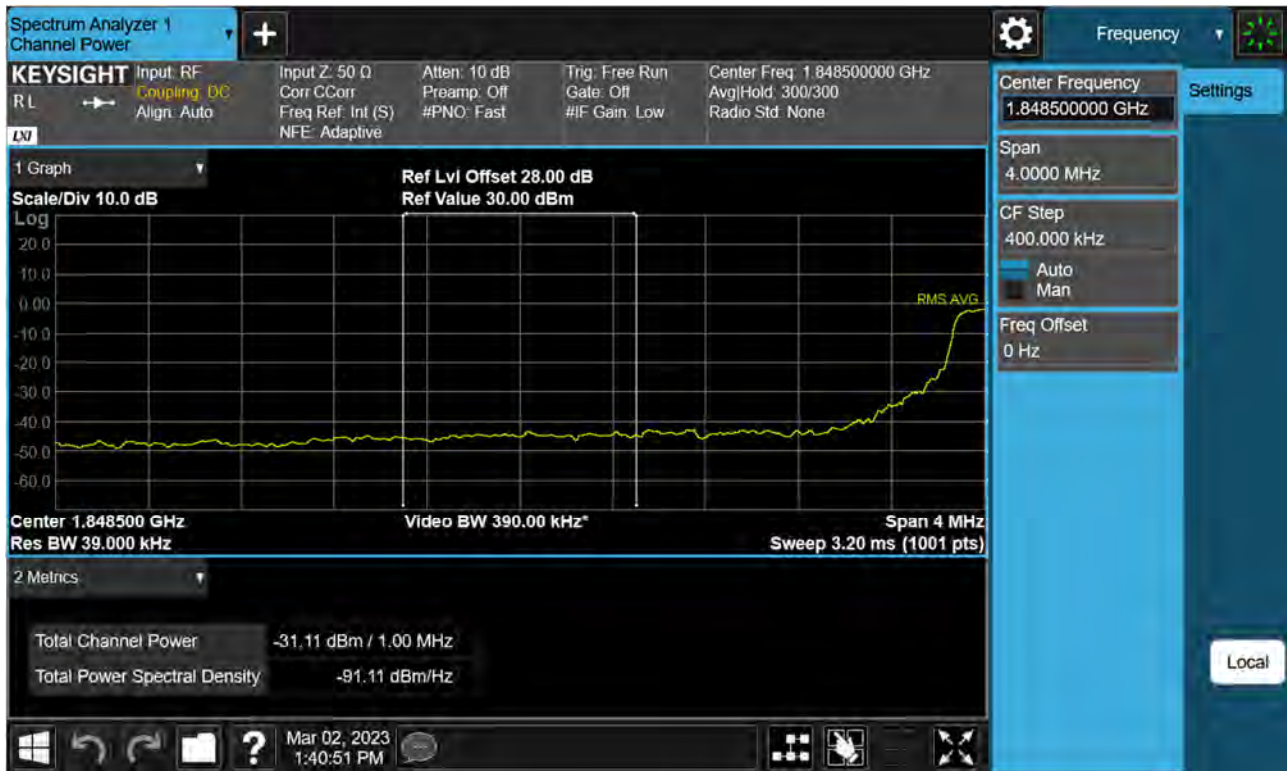
Sub6 n2. Lower Extended Band Edge Plot (15 M BW Ch.371500 BPSK_RB75_0) -3
