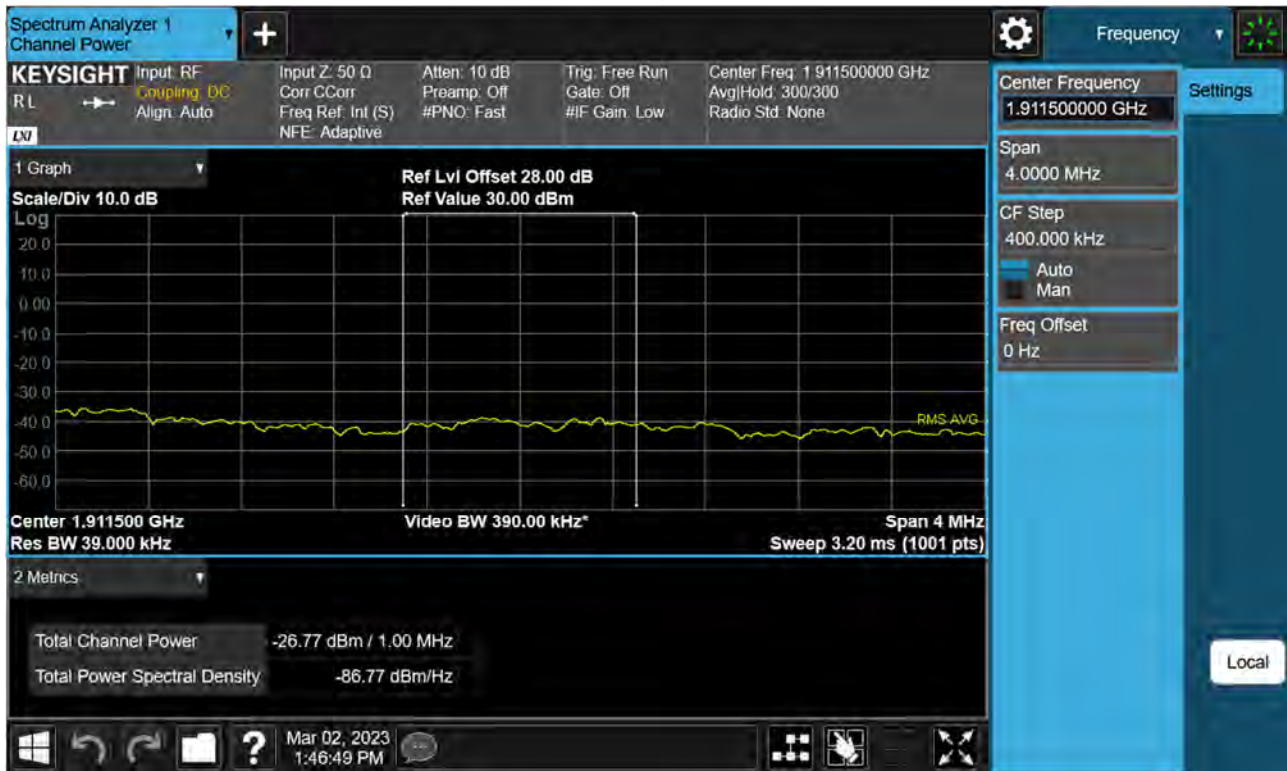
Sub6 n2. Upper Extended Band Edge Plot (20 M BW Ch.380000 BPSK_RB100_0) -3
