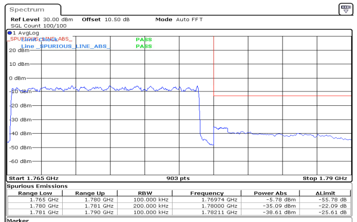
n66_15MHz_15kHz_1772.5MHz_DFT-s-OFDM QPSK_RB75@0
