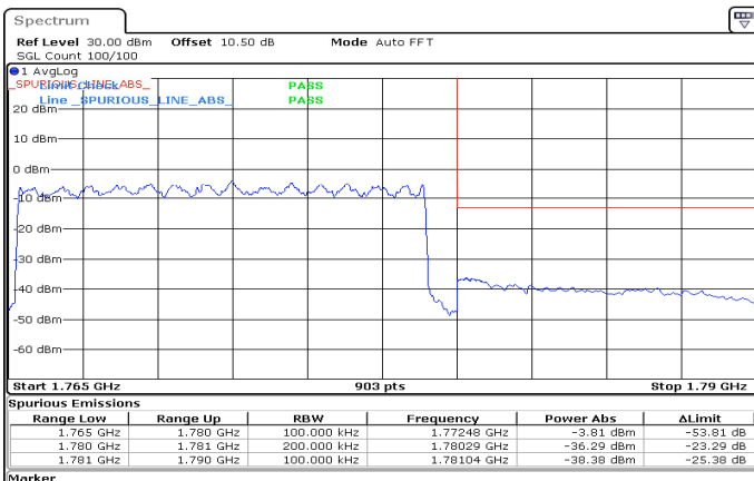
n66_15MHz_15kHz_1772.5MHz_DFT-s-OFDM QPSK_RB1@78
