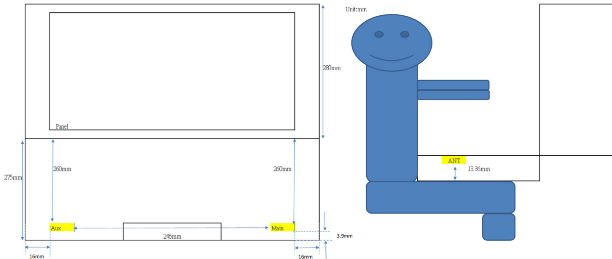
Photograph 7. Antenna position of EUT
