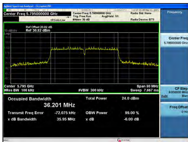
802.11ac(VHT40) (CH.159)
