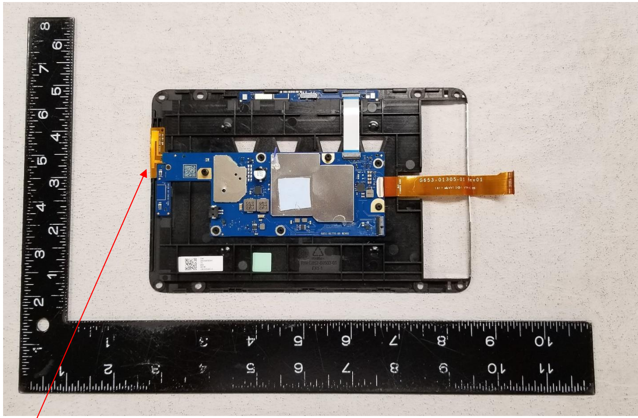
Antenna location
