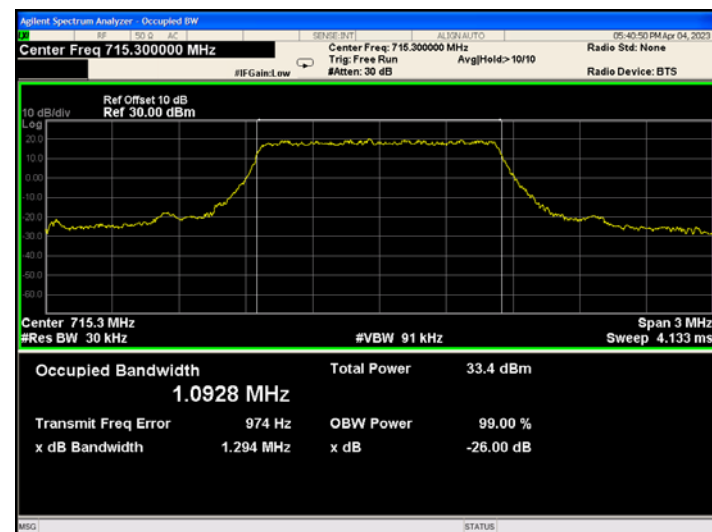
Band12-1.4MHz-QPSK-23173-6RB#0
