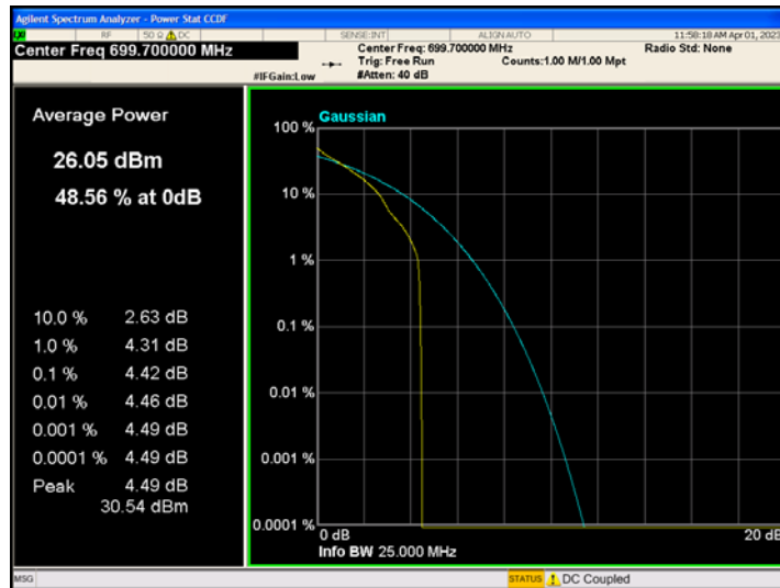
Band12-1.4MHz-QPSK-23017-6RB#0
