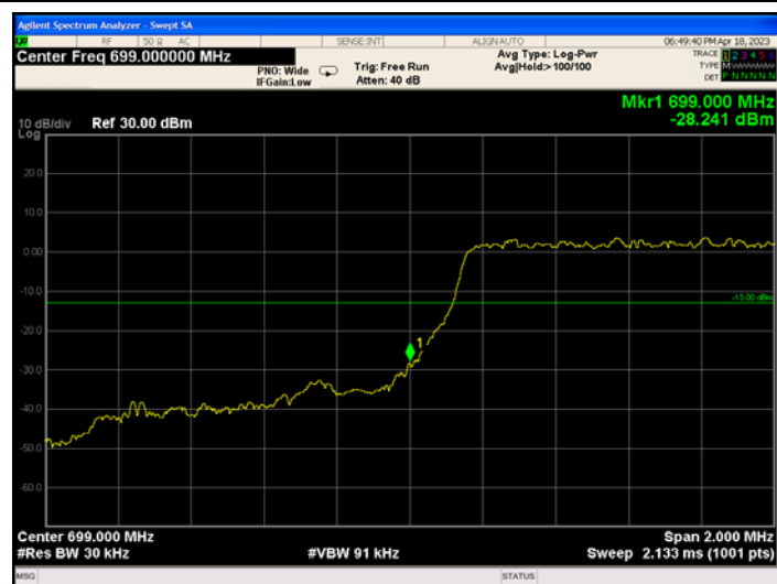
Band12-1.4MHz-QPSK-23017-6RB#0
