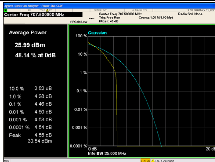
Band12-1.4MHz-QPSK-23095-1RB#0
