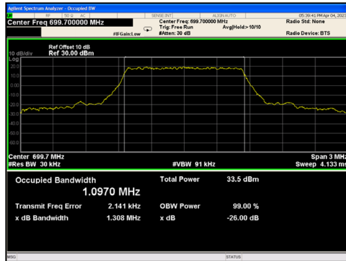
Band12-1.4MHz-QPSK-23095-6RB#0
