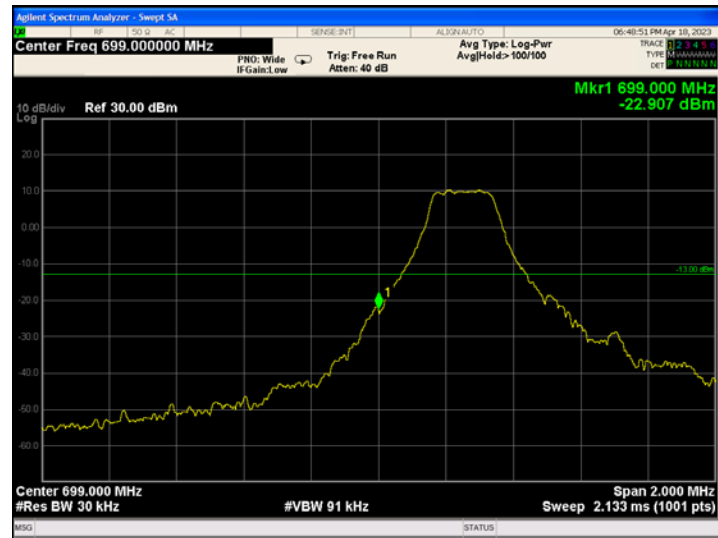
Band12-1.4MHz-QPSK-23017-1RB#5
