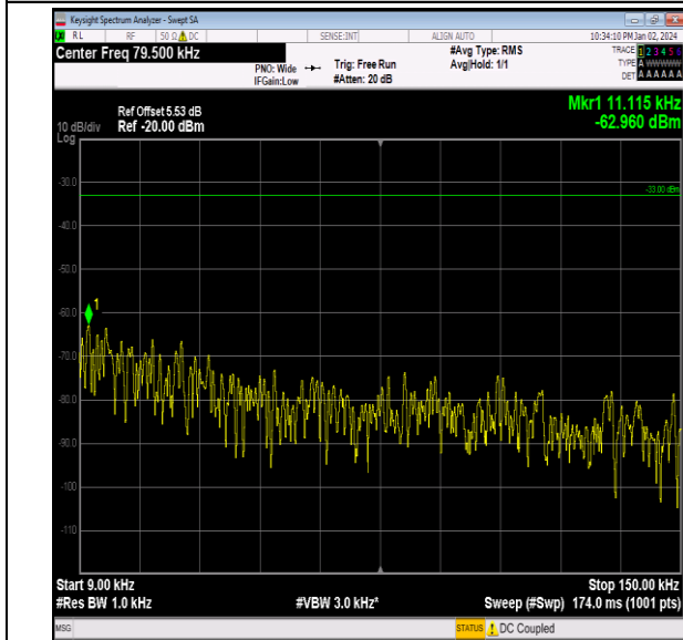
Band26_10MHz_QPSK_26840_1RB#0_0.009~0.15_0.009 ~0.15
