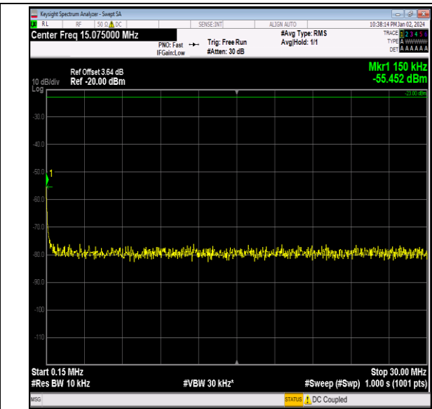
Band26_10MHz_QPSK_26990_1RB#0_0.15~30_0.15~30
