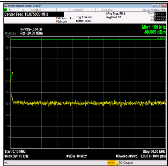
Band26_5MHz_16QAM_26915_1RB#0_0.15~30_0.15~30
