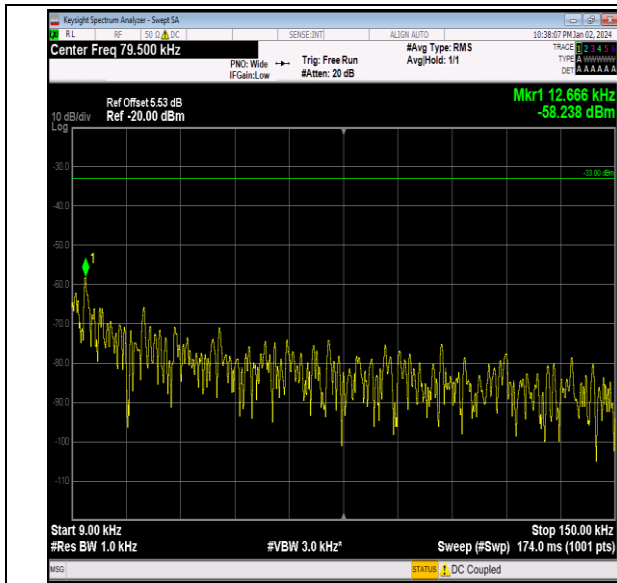
Band26_10MHz_QPSK_26990_1RB#0_0.009~0.15_0.009 ~0.15
