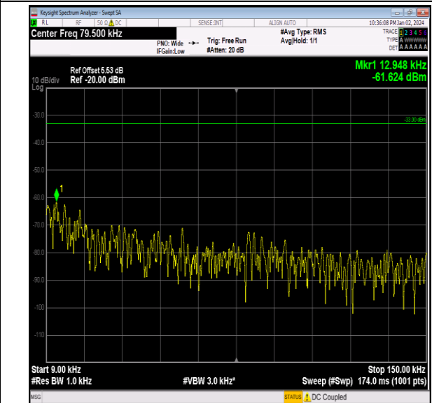
Band26_10MHz_QPSK_26915_1RB#0_0.009~0.15_0.009 ~0.15
