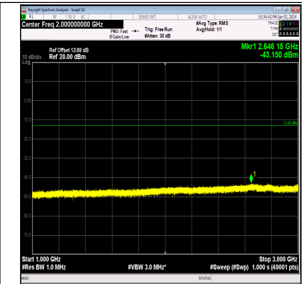
Band26_10MHz_QPSK_26840_1RB#0_1000~3000_1000 ~3000
