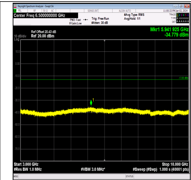
Band26_15MHz_QPSK_26915_1RB#0_3000~10000_300 0~10000
