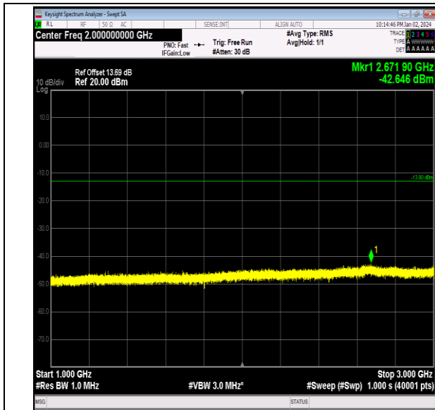
Band26_5MHz_16QAM_27015_1RB#0_1000~3000_1000 ~3000
