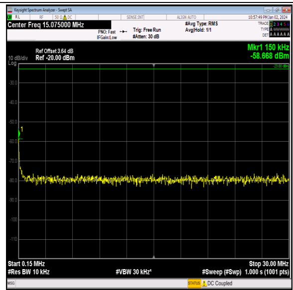
Band26_15MHz_QPSK_26865_1RB#0_0.15~30_0.15~30
