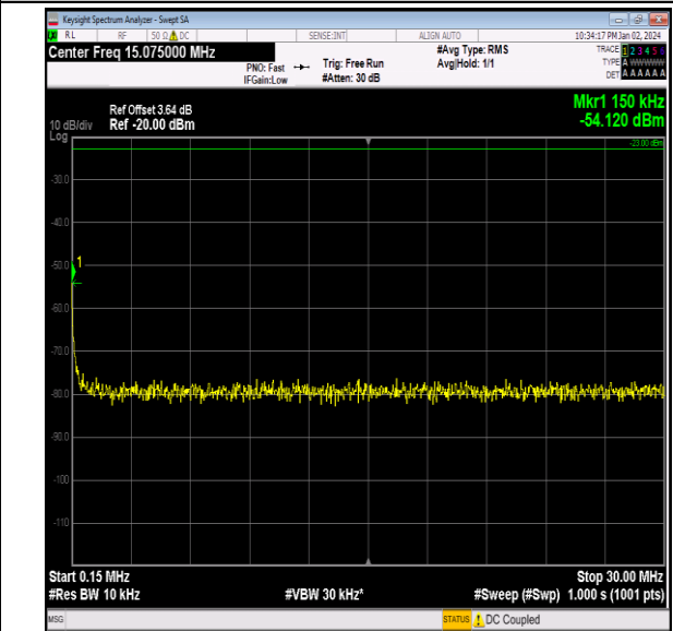
Band26_10MHz_QPSK_26840_1RB#0_0.15~30_0.15~30
