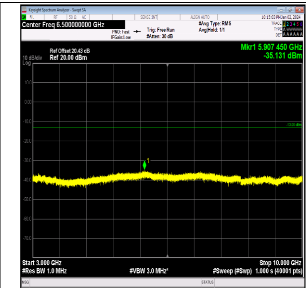
Band26_5MHz_16QAM_27015_1RB#0_3000~10000_300 0~10000
