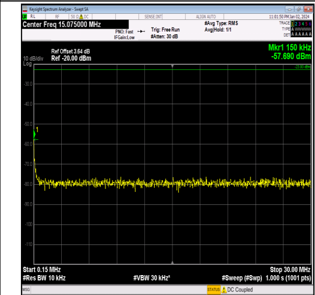
Band26_15MHz_QPSK_26965_1RB#0_0.15~30_0.15~30
