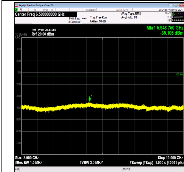
Band26_10MHz_QPSK_26840_1RB#0_3000~10000_300 0~10000
