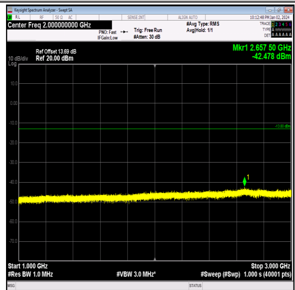
Band26_5MHz_16QAM_26915_1RB#0_1000~3000_1000 ~3000
