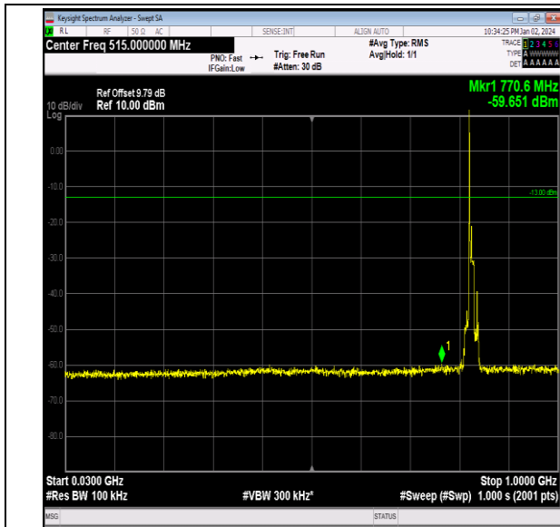
Band26_10MHz_QPSK_26840_1RB#0_30~1000_30~100 0
