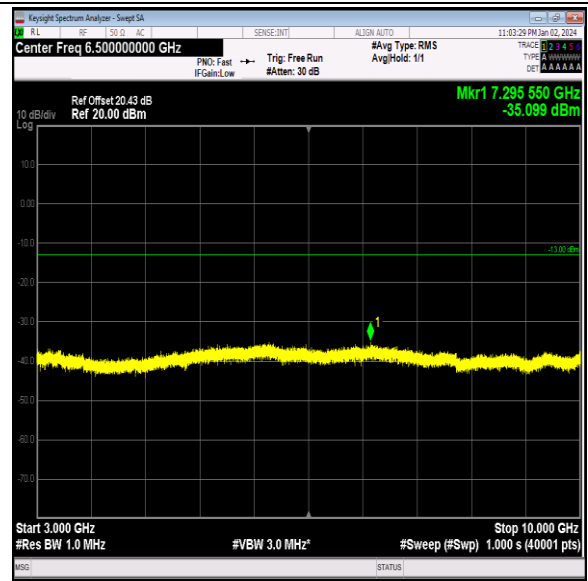
Band26_15MHz_16QAM_26965_1RB#0_3000~10000_30 00~10000
