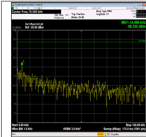
Band26_5MHz_16QAM_26915_1RB#0_0.009~0.15_0.009 ~0.15
