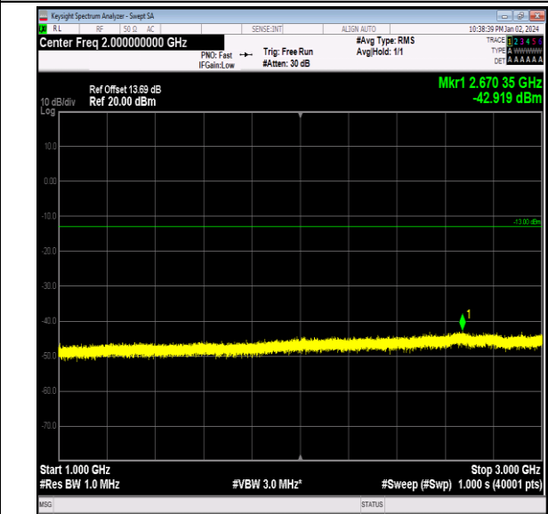
Band26_10MHz_QPSK_26990_1RB#0_1000~3000_1000 ~3000
