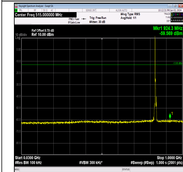
Band26_5MHz_16QAM_26915_1RB#0_30~1000_30~100 0
