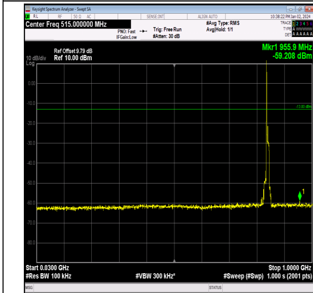
Band26_10MHz_QPSK_26990_1RB#0_30~1000_30~100 0
