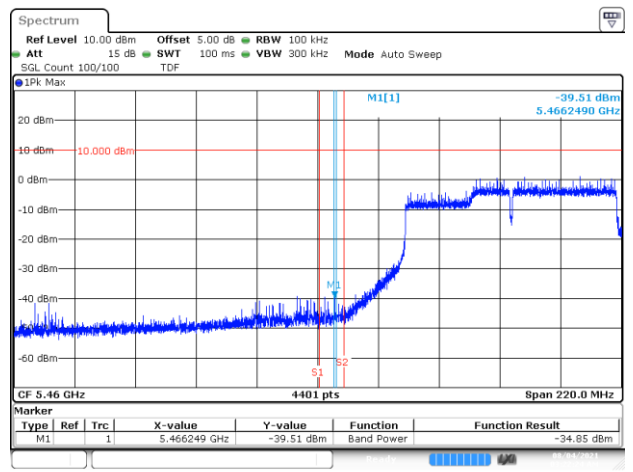
BE-NR-LOW, MIMO-B, 802.11ac160-VHT0, Ch114
