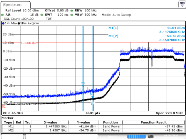
BE-R-LOW, MIMO-B, 802.11ac80-VHT0, Ch106
