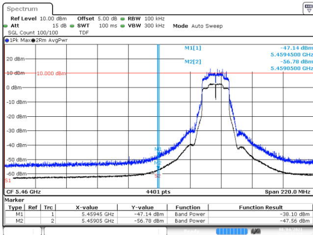
BE-R-LOW, MIMO-B, 802.11ax20-HE0, Ch100
