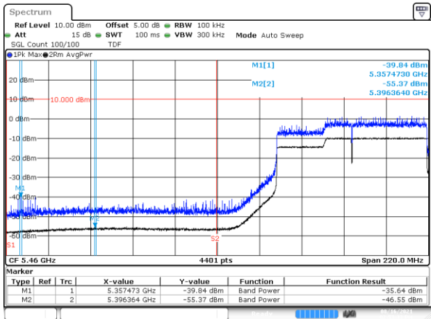
BE-R-LOW, SISO-A, 802.11ax160-HE0, Ch114
