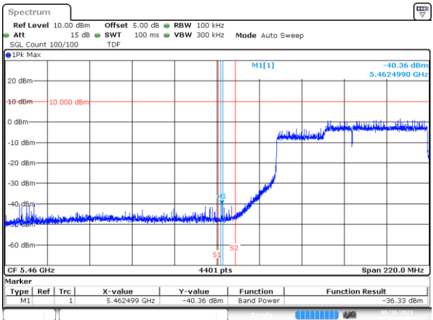
BE-NR-LOW, SISO-A, 802.11ax160-HE0, Ch114
