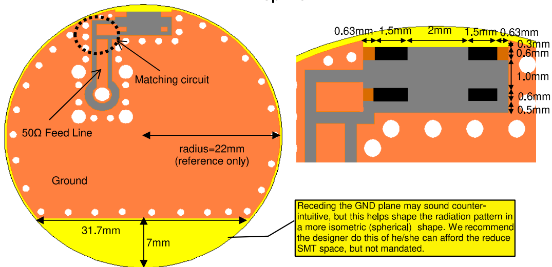
Bottom View
