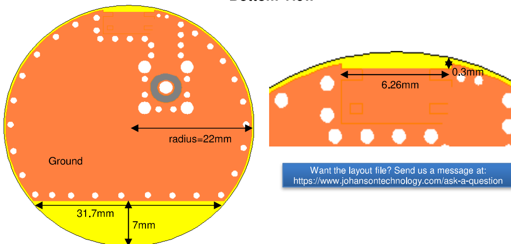
Bottom View
