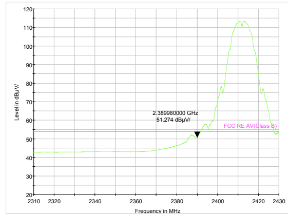
802.11b-Channel 1 Average
