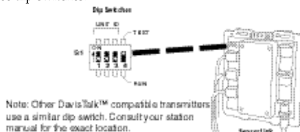
TRANSMITTER DIP-SWITCHES
