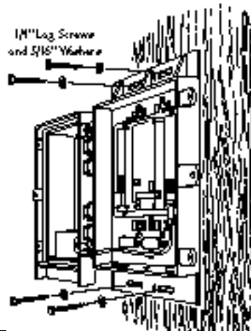
MOUNTING SOLAR POWERED REPEATER ON A WALL OR POST
