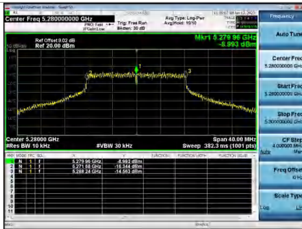
Freq. Stability 0C 120V a 5280MHz Ant1 0 Minutes
