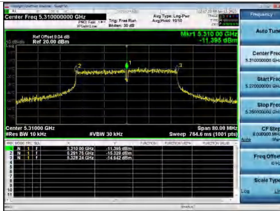
Freq. Stability 50C 120V n40 5310MHz Ant1 0 Minutes
