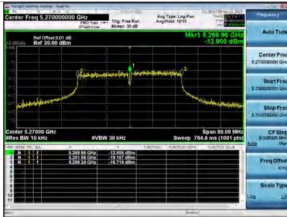
Freq. Stability 0C 120V ac40 5270MHz Ant1 0 Minutes
