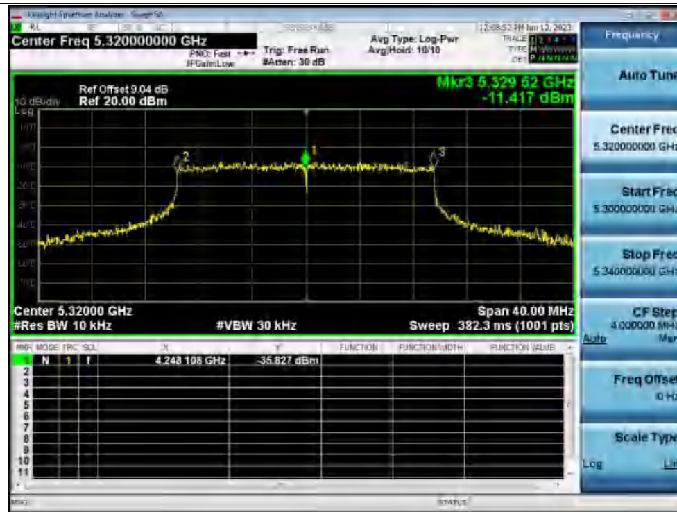
Freq. Stability 20C 120V ax20 5320MHz Ant1 0 Minutes
