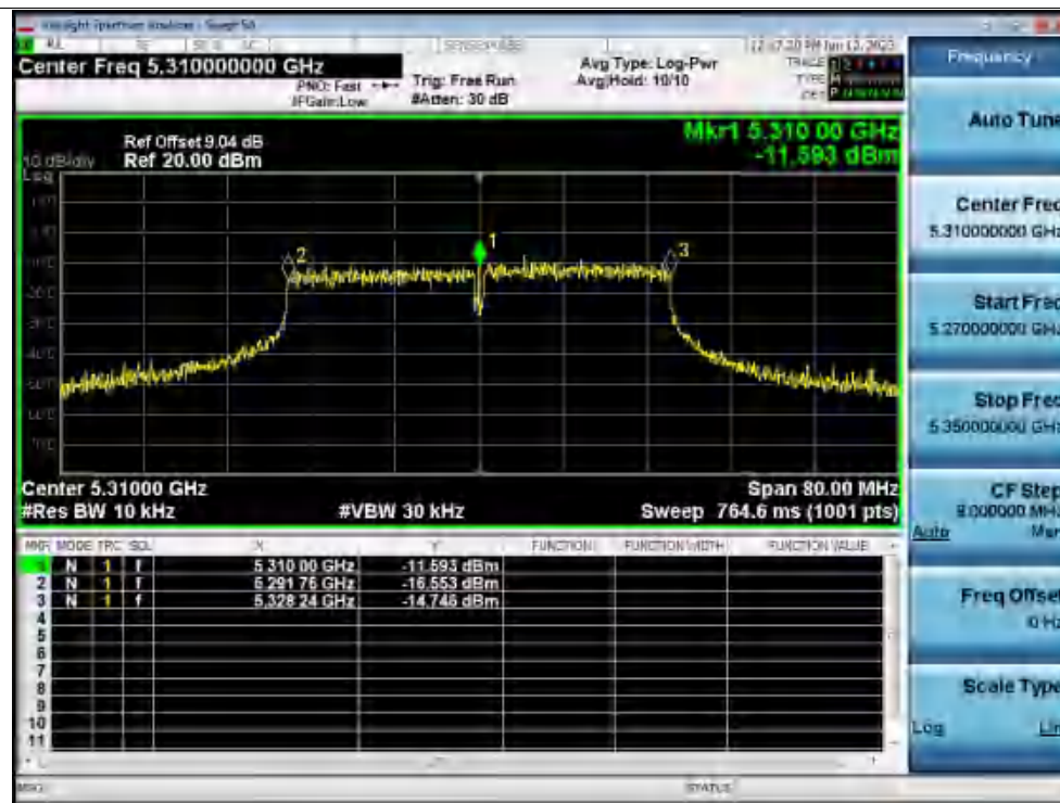
Freq. Stability 30C 120V n40 5310MHz Ant1 0 Minutes
