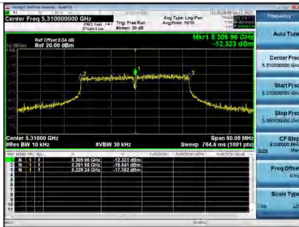
Freq. Stability 30C 120V ac40 5310MHz Ant1 0 Minutes
