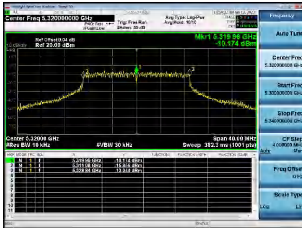
Freq. Stability 0C 120V ac20 5320MHz Ant1 0 Minutes
